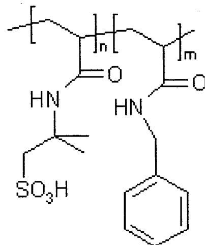
AMPS- BzAAm copolymer
