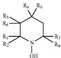
1-alkoxy-2,2,6,6-tetraalkylpiperidines of the formula
