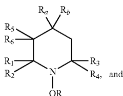
1-acyloxy-2,2,6,6-tetraalkylpiperidines of the formula
