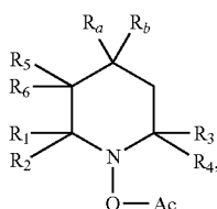
1-acyloxy-2,2,6,6-tetraalkylpiperidines of the formula
