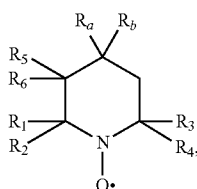
1-hydroxy-2,2,6,6-tetraalkylpiperidines of the formula
