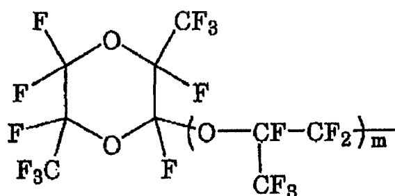
[Chem. 1]
