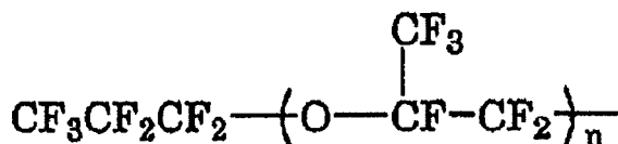
[Chem. 2]
