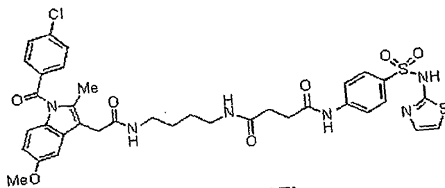
Compound 27j
