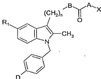
Formula III,
