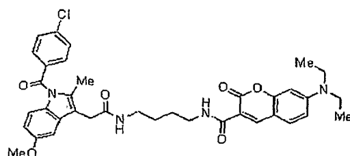
Compound 27ff
