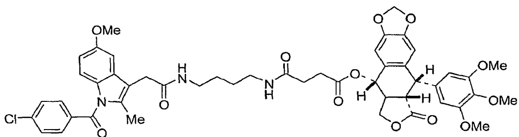
Compound 27n
