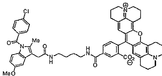
Compound 27eee
