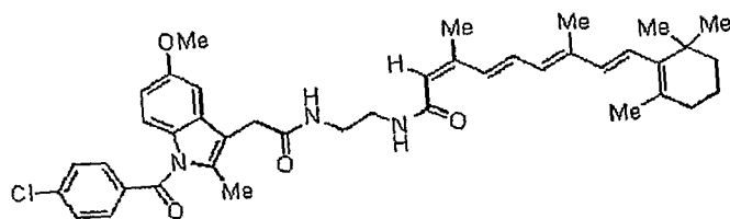
Compound 27g
