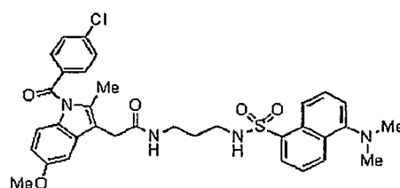
Compound 27y
