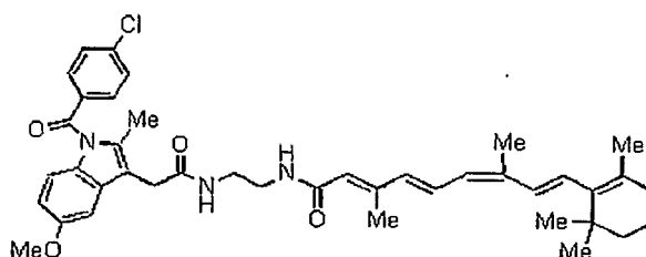
Compound 27s
