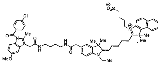
Compound 27qqq
