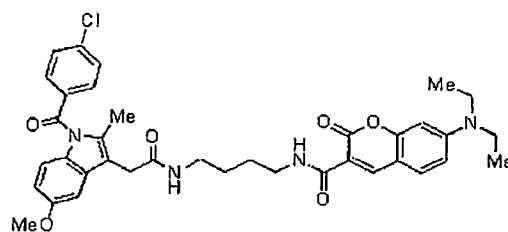
Compound 27ff
