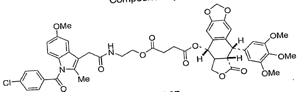
Compound 27q
