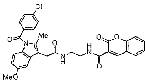
Compound 27cc
