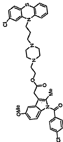
Perphenazine Analog
