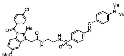
Compound 27aa
