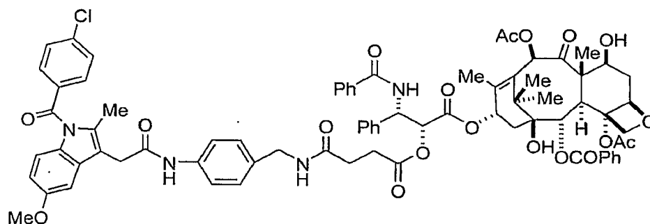
Compound 27d
