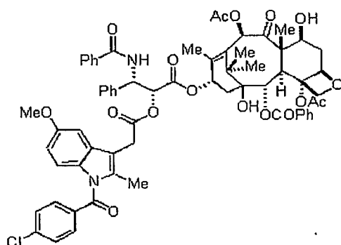
Compound 27a
