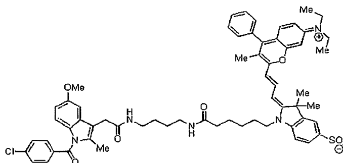
Compound 27ttt
