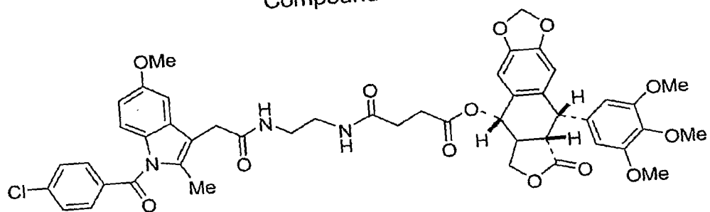
Compound 27o
