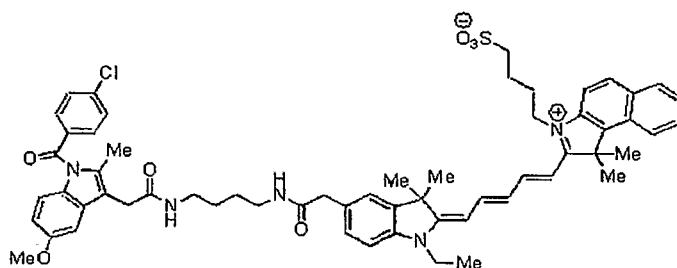
Compound 27qqq
