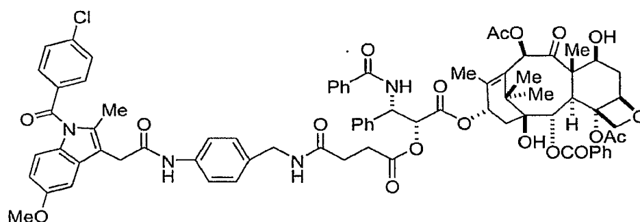
Compound 27d
