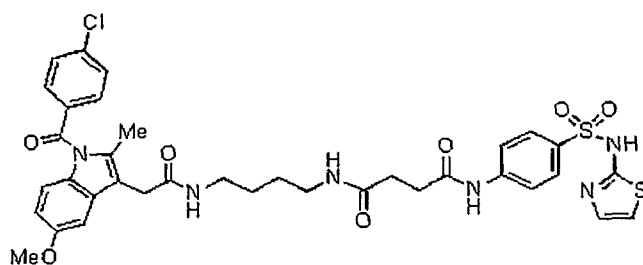
Compound 27j
