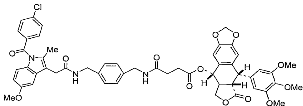
Compound 27r
