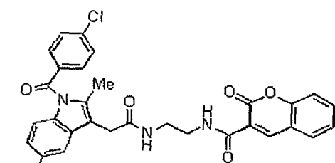
Compound 27cc
