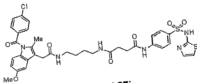
Compound 27j
