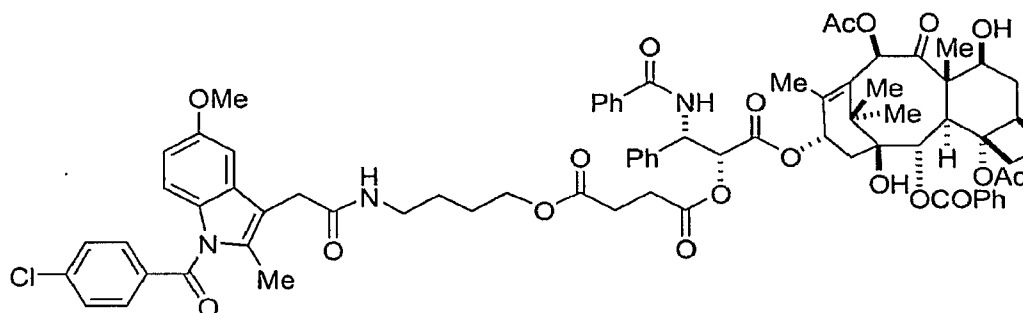
Compound 27c
