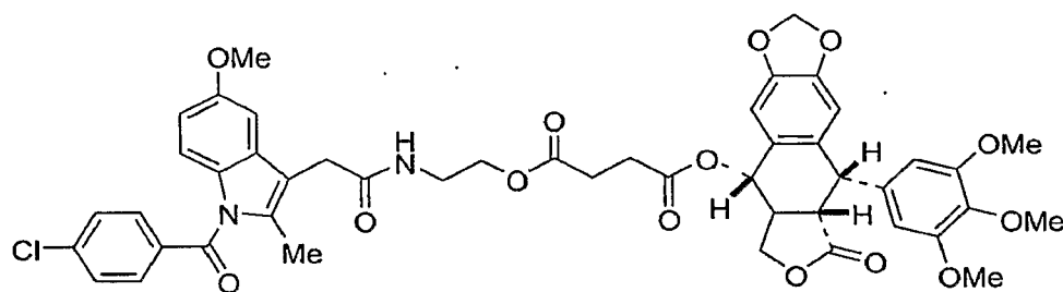
Compound 27q
