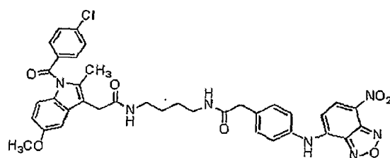
Compound 27ii
