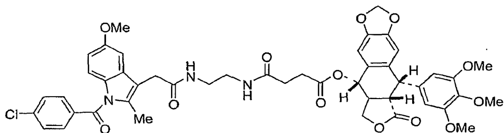
Compound 27o
