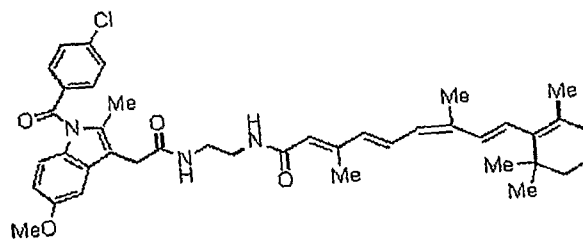
Compound 27s
