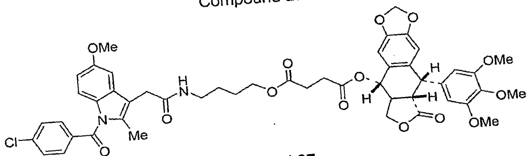
Compound 27p
