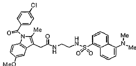
Compound 27x
