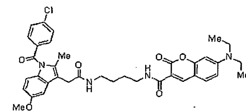
Compound 27ff
