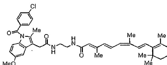
Compound 27s
