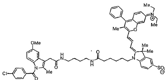
Compound 27ttt
