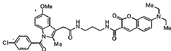
Compound 27gg
