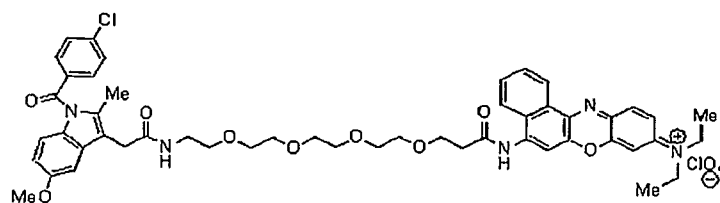
Compound 27uu
