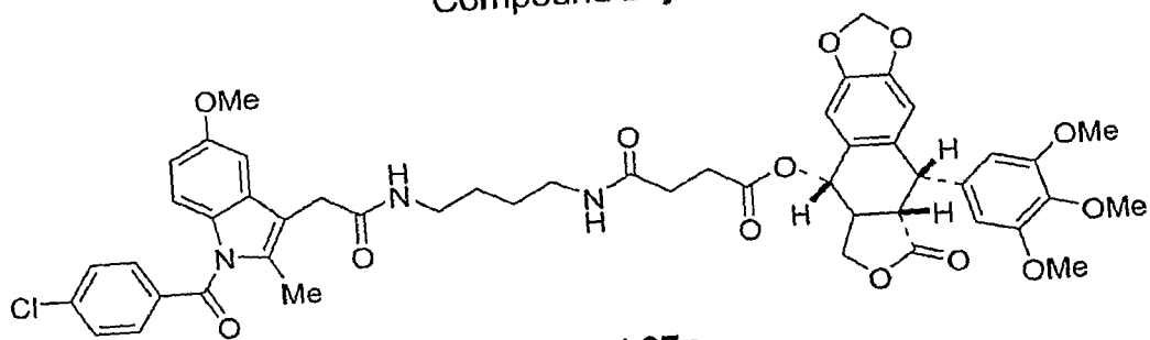
Compound 27n
