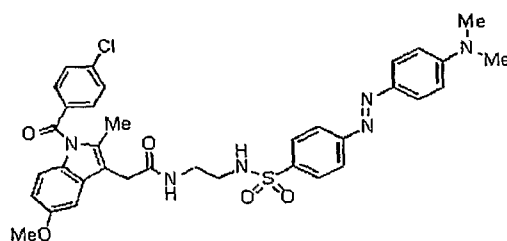
Compound 27aa
