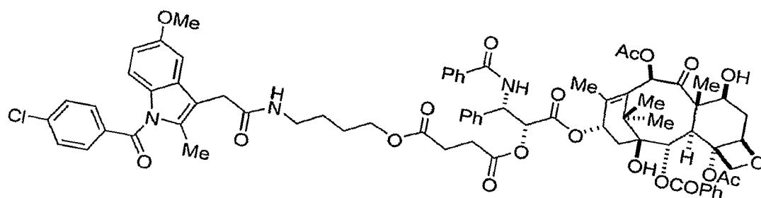
Compound 27c
