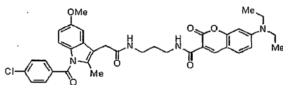
Compound 27ff
