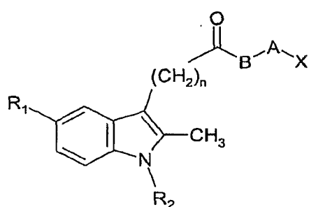
Formula I,
