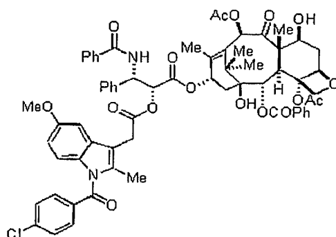
Compound 27a
