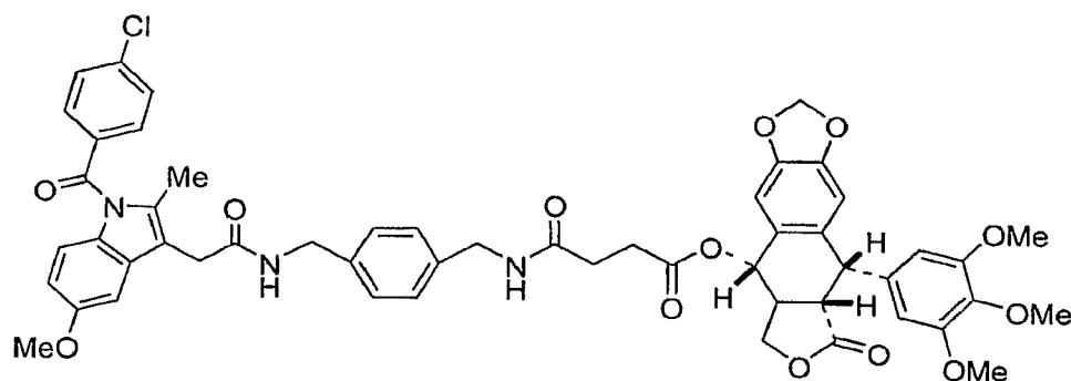
Compound 27r
