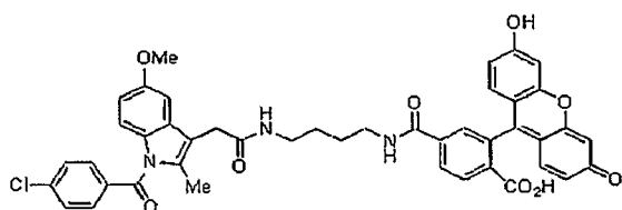
Compound 27qq
