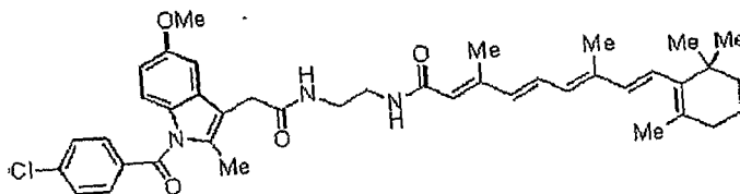
Compound 27h
