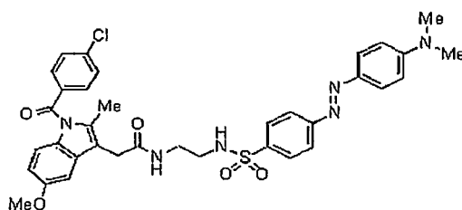
Compound 27aa
