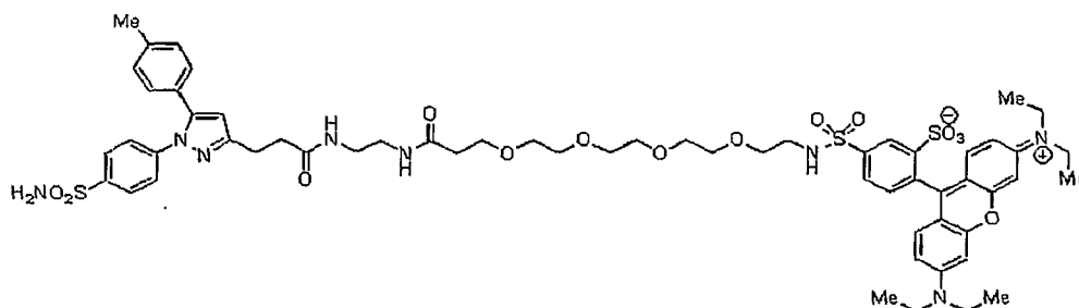
Compound 30f
