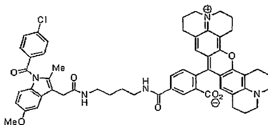
Compound 27eee
