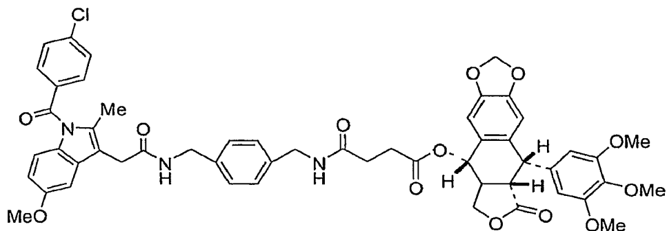
Compound 27r
