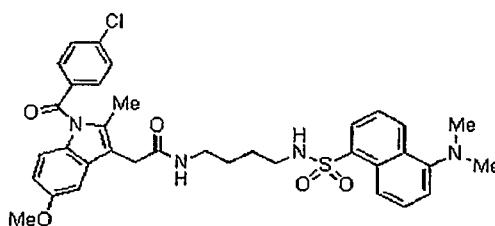
Compound 27z
