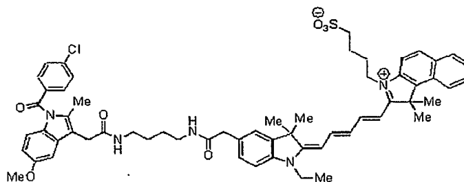
Compound 27qqq
