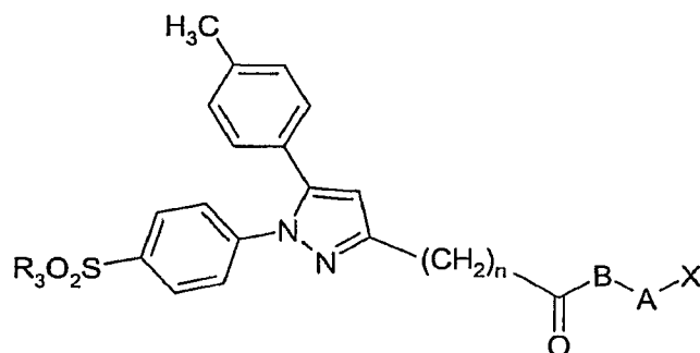
Formula III,
