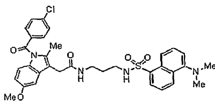
Compound 27y
