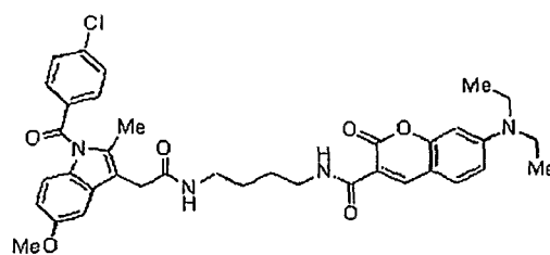
Compound 27ff
