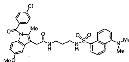
Compound 27y
