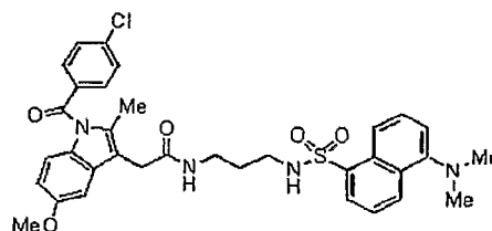
Compound 27y
