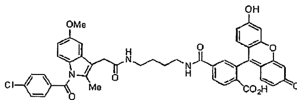
Compound 27pp
