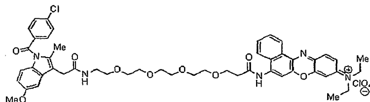
Compound 27uu
