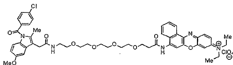
Compound 27uu
