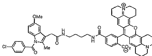
Compound 27vv
