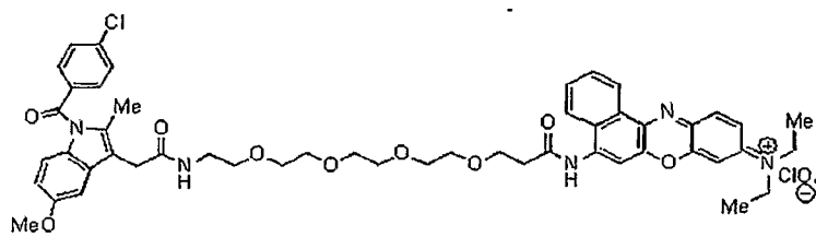
Compound 27uu
