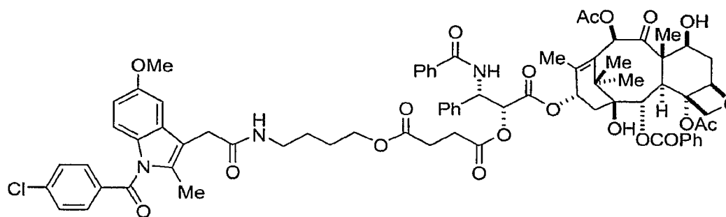
Compound 27c
