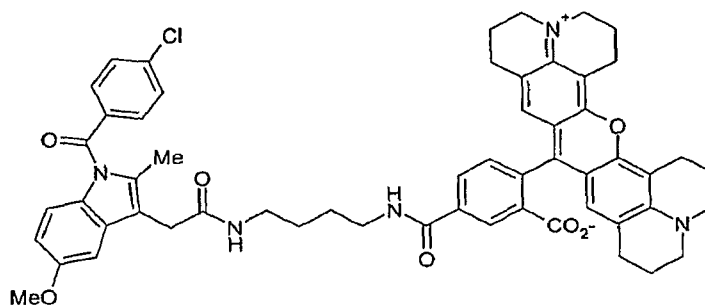
Compound 27eee
