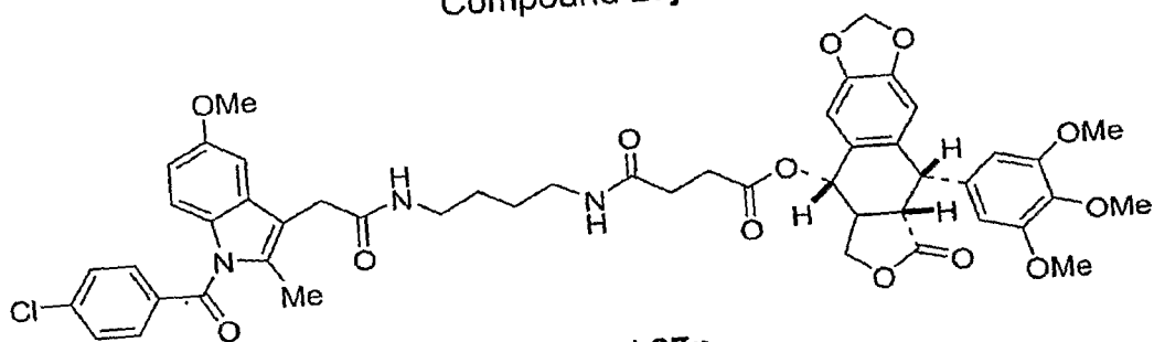
Compound 27n
