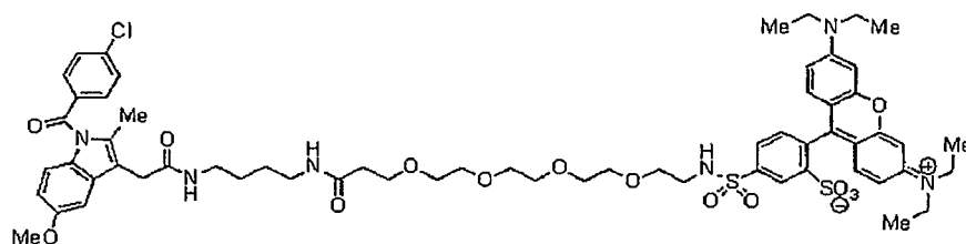
Compound 27iii
