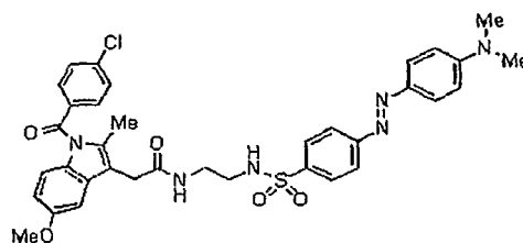
Compound 27aa
