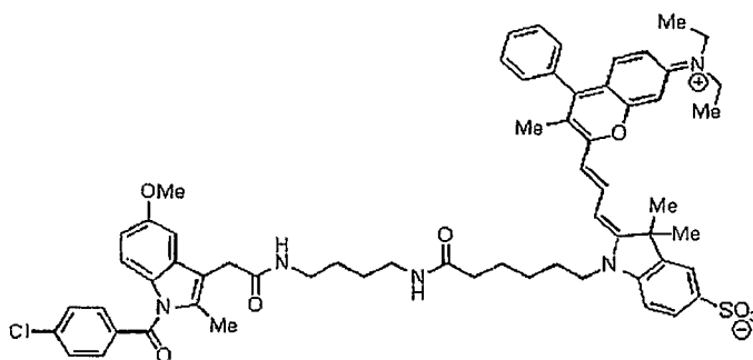
Compound 27ttt
