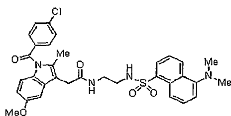
Compound 27x
