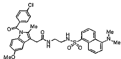
Compound 27x
