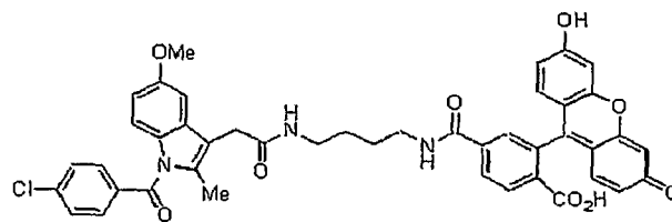
Compound 27qq
