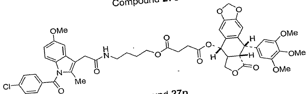
Compound 27p
