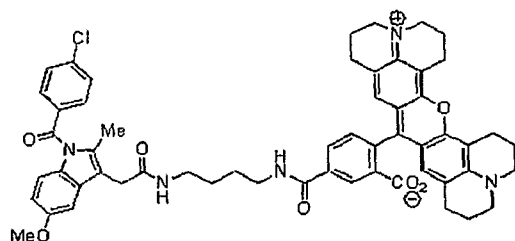
Compound 27eee
