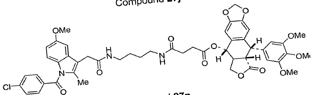
Compound 27n
