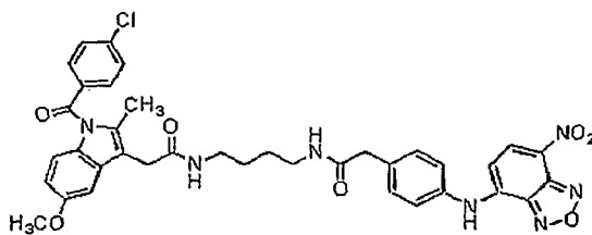
Compound 27ii
