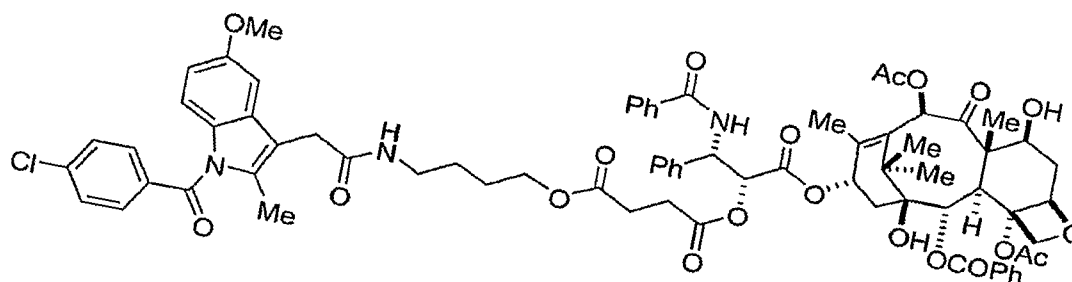
Compound 27c
