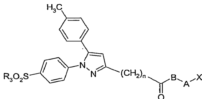
Formula III,
