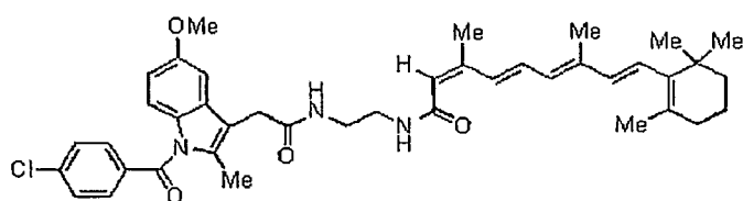
Compound 27g
