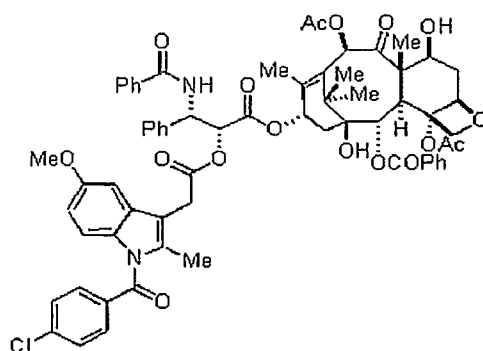
Compound 27a
