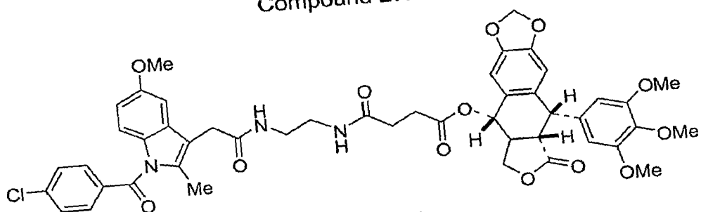
Compound 27o
