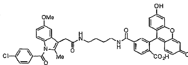
Compound 27qq
