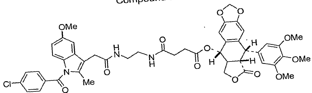
Compound 27o
