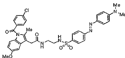
Compound 27aa
