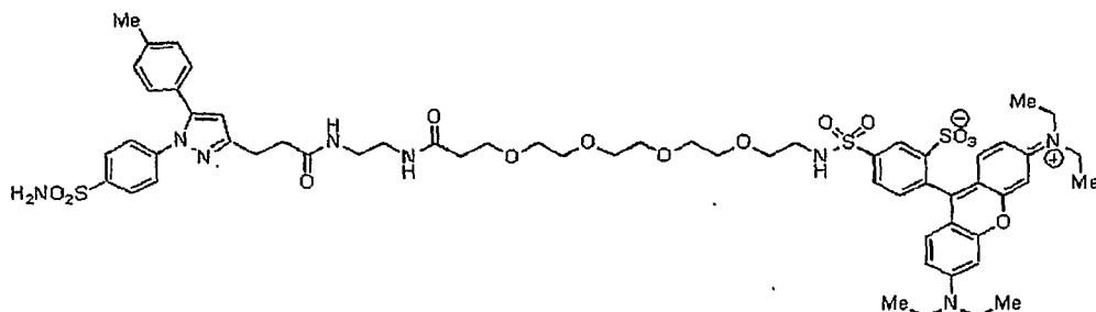
Compound 30f
