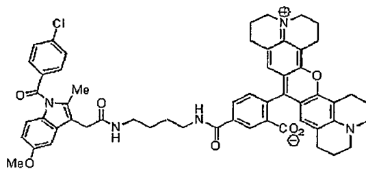
Compound 27eee
