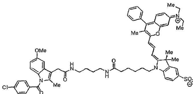
Compound 27w
