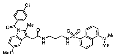
Compound 27y
