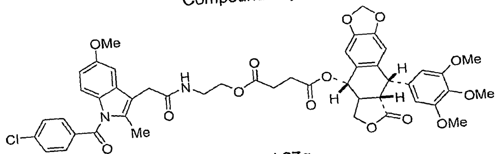
Compound 27q
