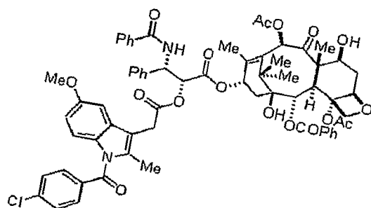
Compound 27a
