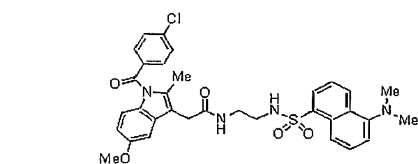
Compound 27x
