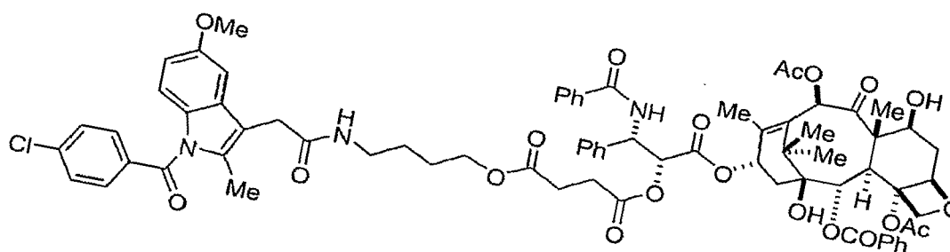
Compound 27c
