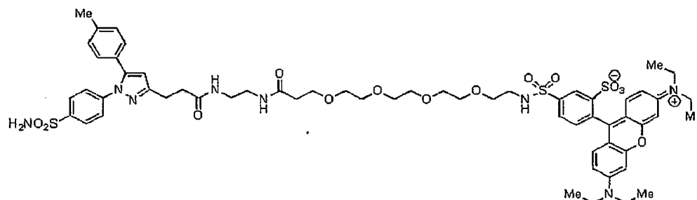
Compound 30f
