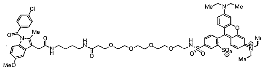
Compound 27iii
