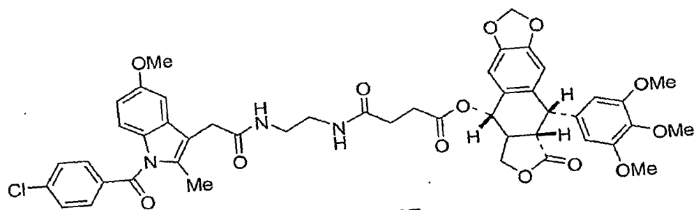
Compound 27o
