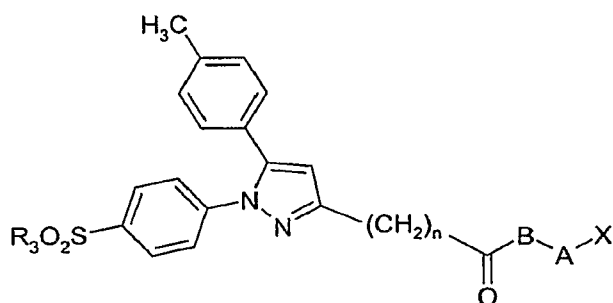
Celecoxib Analog
