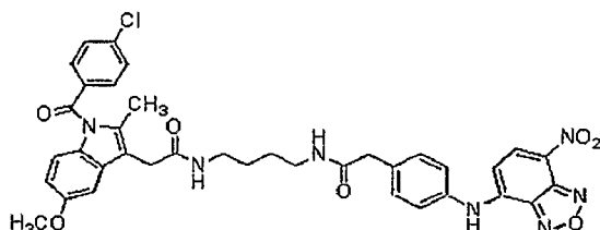
Compound 27ii
