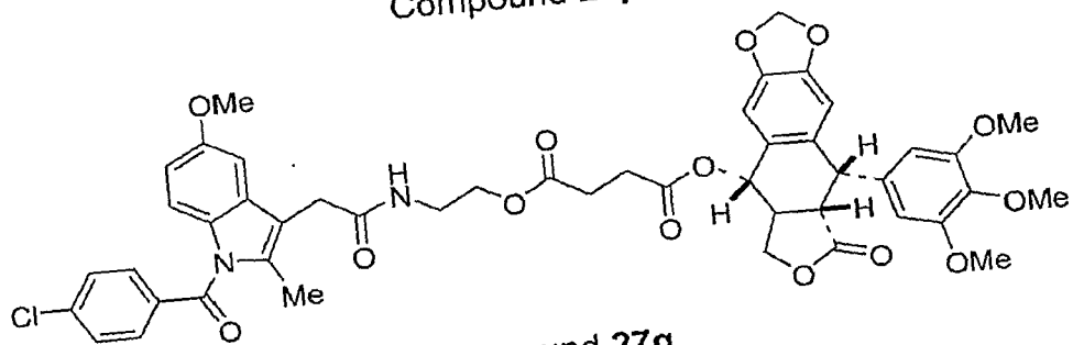
Compound 27q
