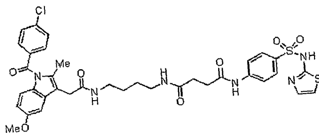
Compound 27j
