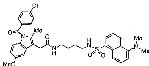
Compound 27z
