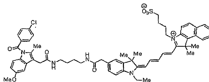
Compound 27qqq
