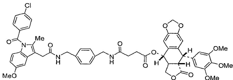
Compound 27r
