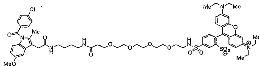
Compound 27iii
