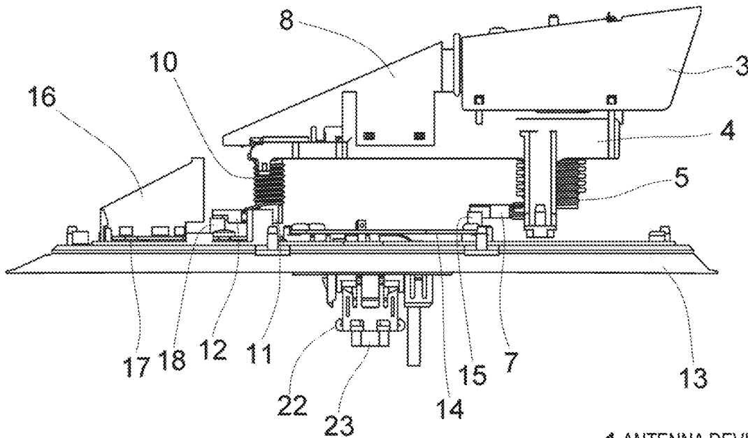
1 ANTENNA DEVICE
