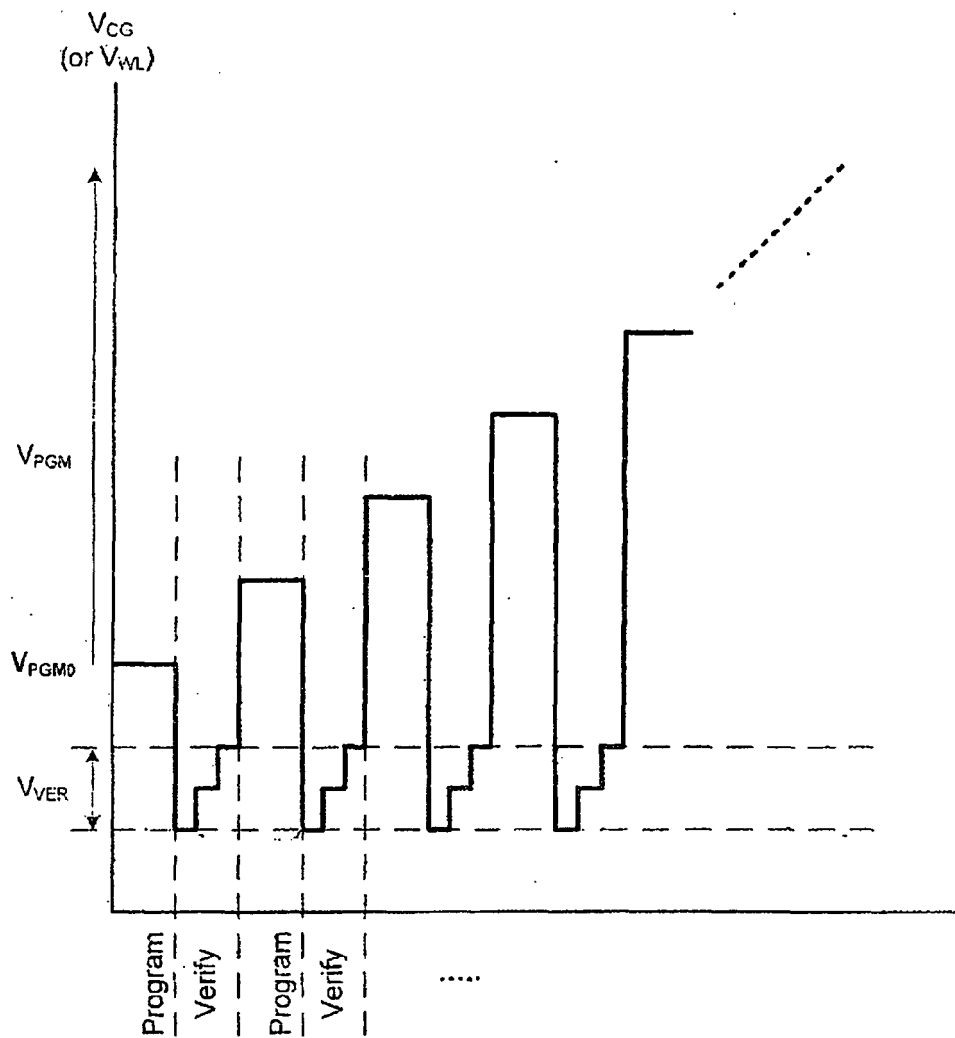
Convention Programming with alternate Program/Verify sequence
