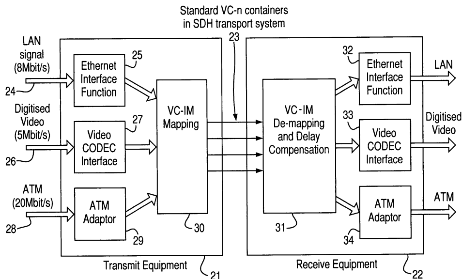
Examples of VC-IM carrying Broadband Signals over an SDH Network
