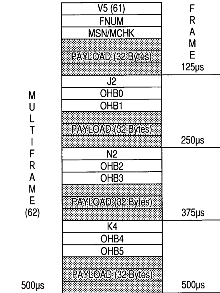
Fig.5. VC-IM-12 Interface Signal Format
