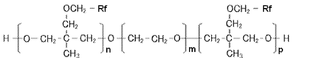
Structural Formula (II)
