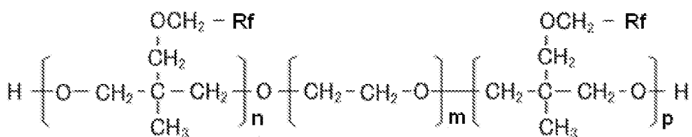
Structural Formula (II)
