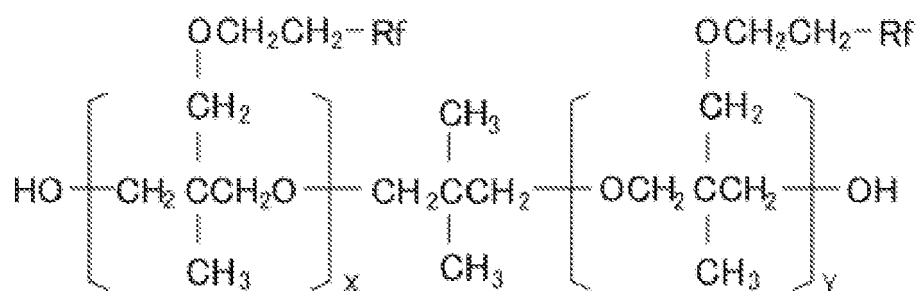
Structural Formula (I)
