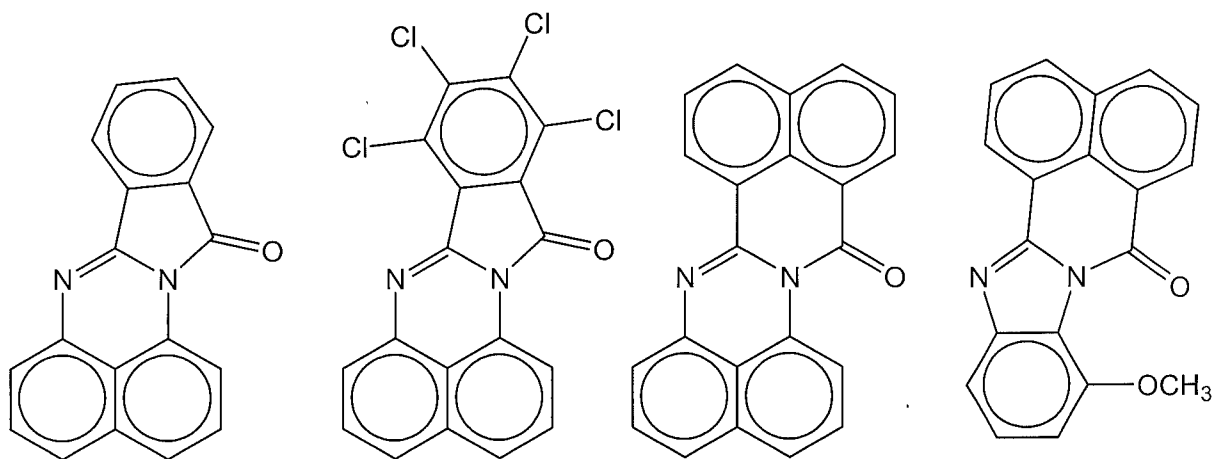
Solvent Orange 60
