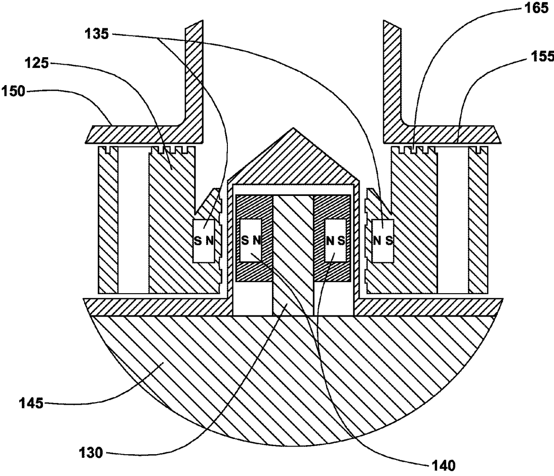
FIG. 13 (DETAIL D)
