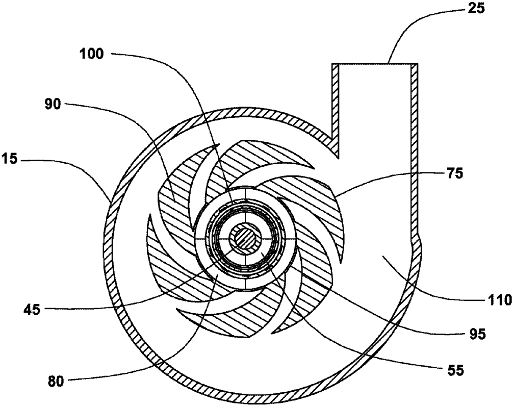
FIG. 3 (SECTION B - B)
