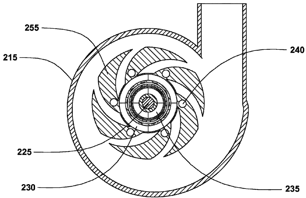
FIG. 19 (Section G-G)
