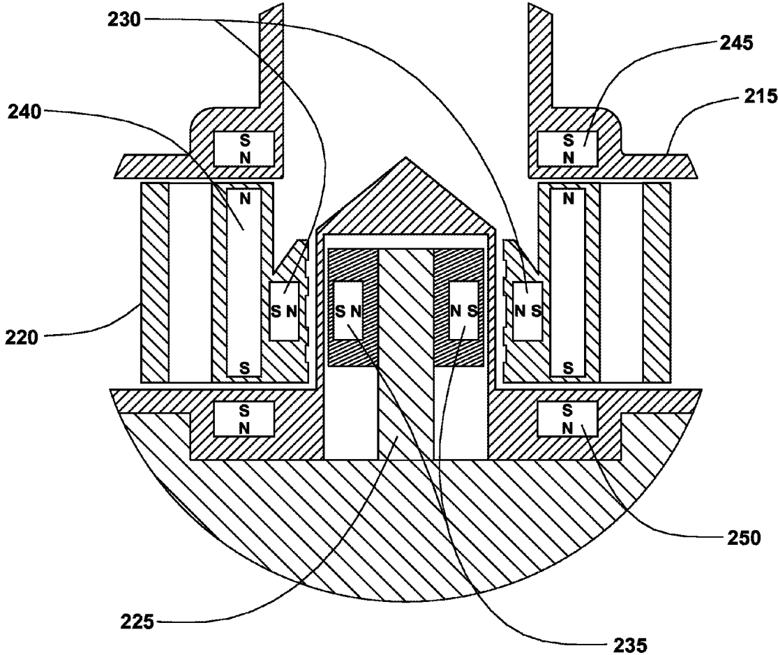
FIG.20 (DETAIL H)
