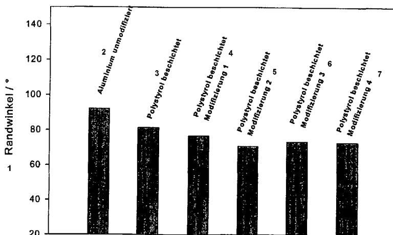
1 WETTING ANGLE 2 ALUMINUM NOT MODIFIED 3 COATED POLYSTYRENE 4 MODIFICATION 1 5 MODIFICATION 2 6 MODIFICATION 3 7 MODIFICATION 4
