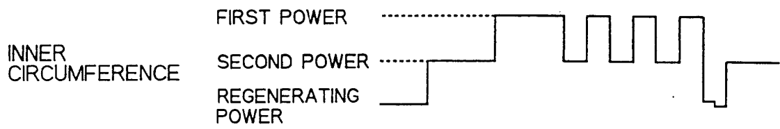
RECORDING WAVEFORM 17-2
