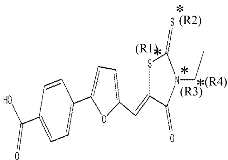
4{5-[(3-ethyl-4-oxo-2-thioxo-1,3-thiazolidin-5-ylidene)methyl]-2-furyl} benzoic acid
