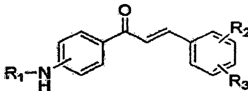
[Chemical Formula 1]
