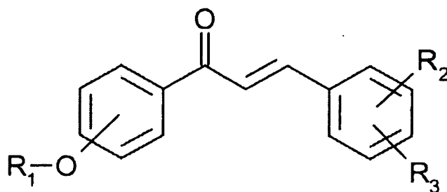
[Chemical Formula 2]
