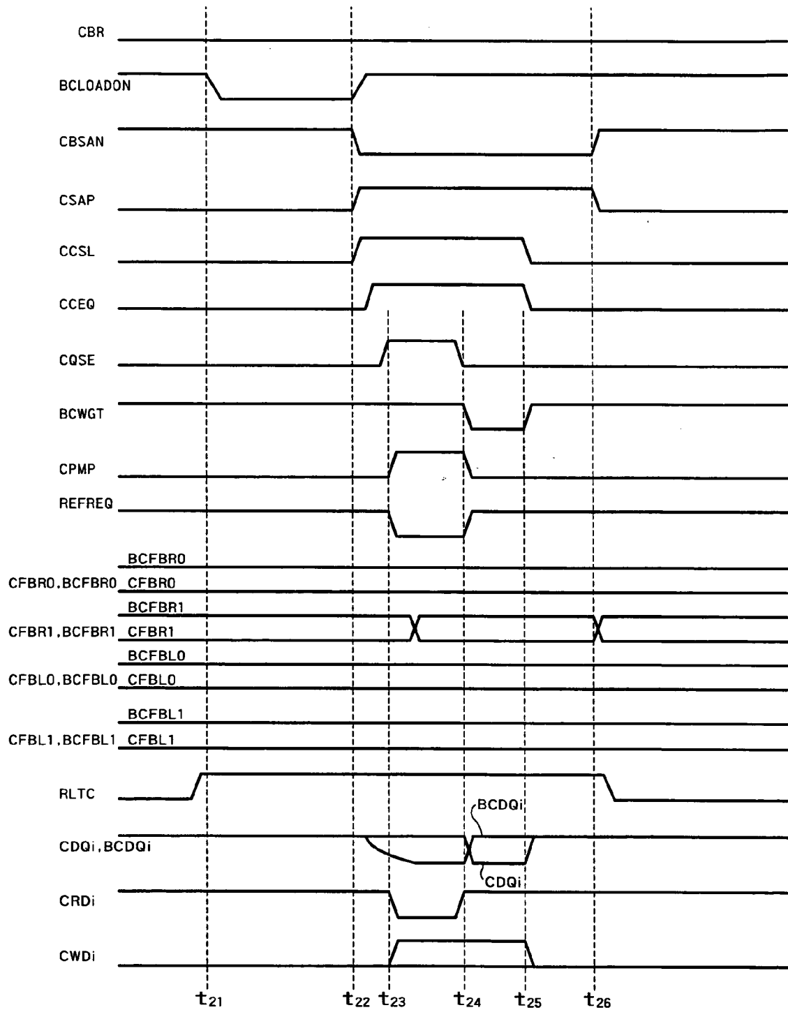
READ/WRITE OPERATION, WITH AD HOC REFRESH OPERATION
