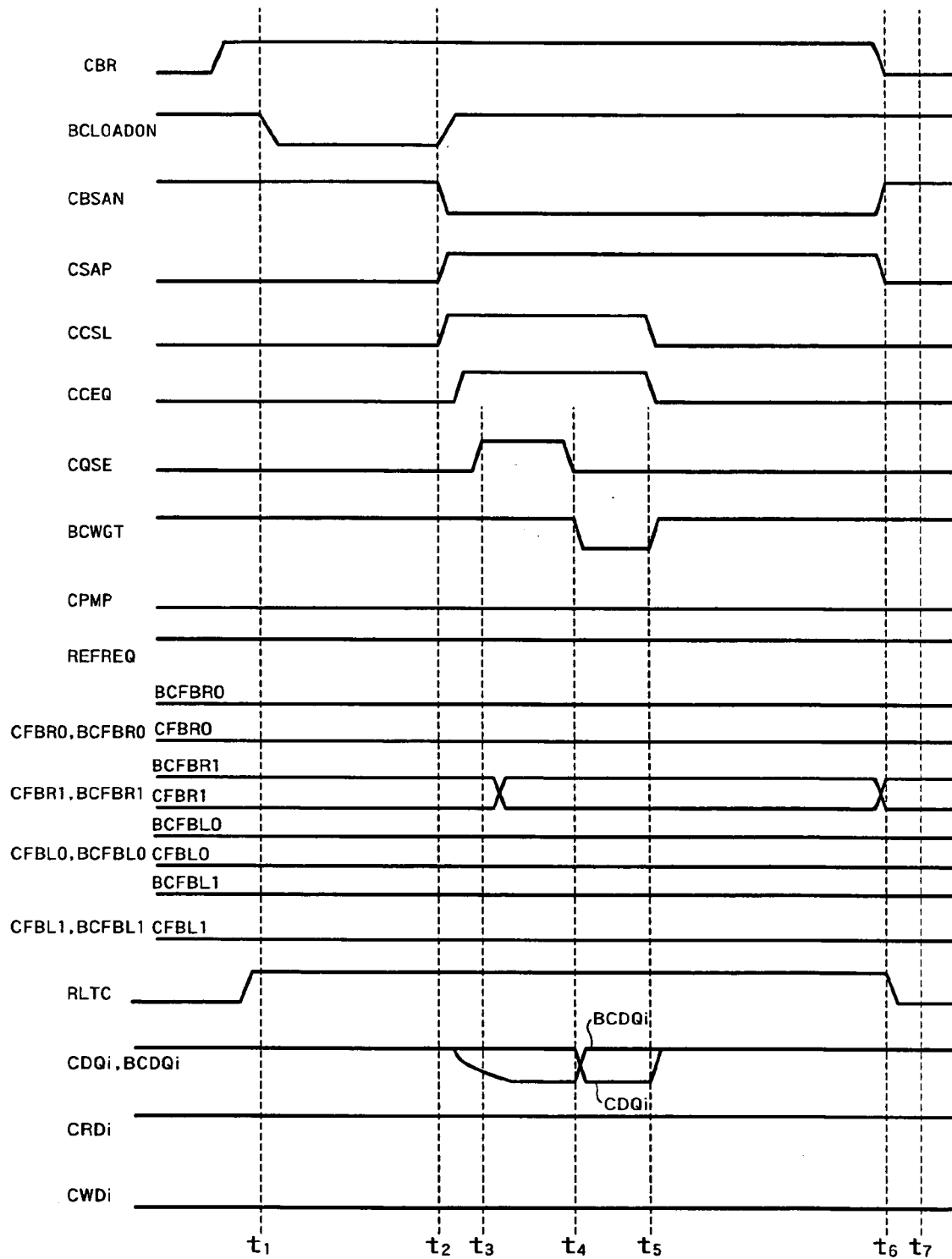
NORMAL REFRESH OPERATION
