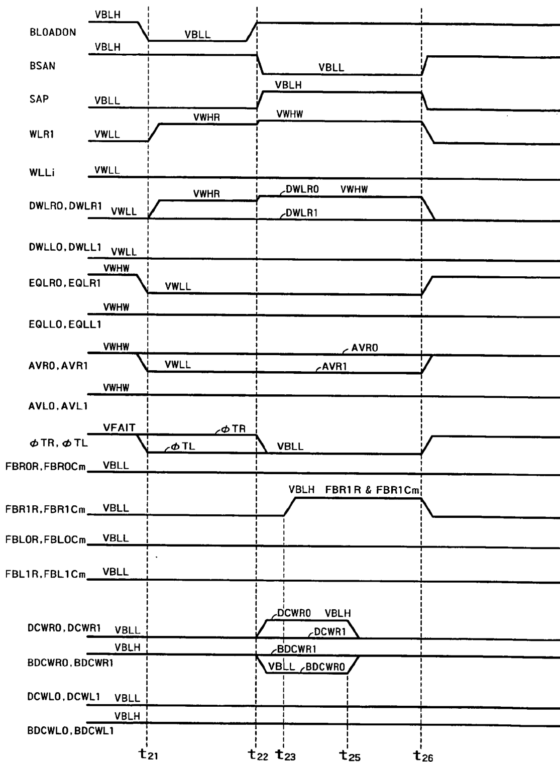
READ/WRITE OPERATION, WITH AD HOC REFRESH OPERATION
