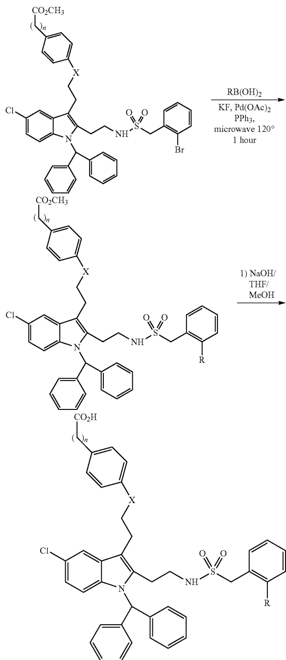
Method B: Suzuki Method
