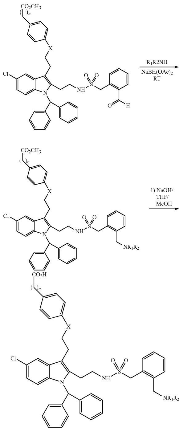
Method C: Reductive Amination Method
