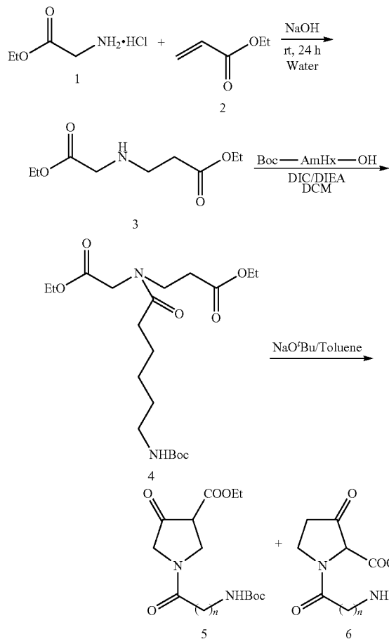
Scheme 1. Synthesis of cis-(3S,4R)-pyrrolidine diol
