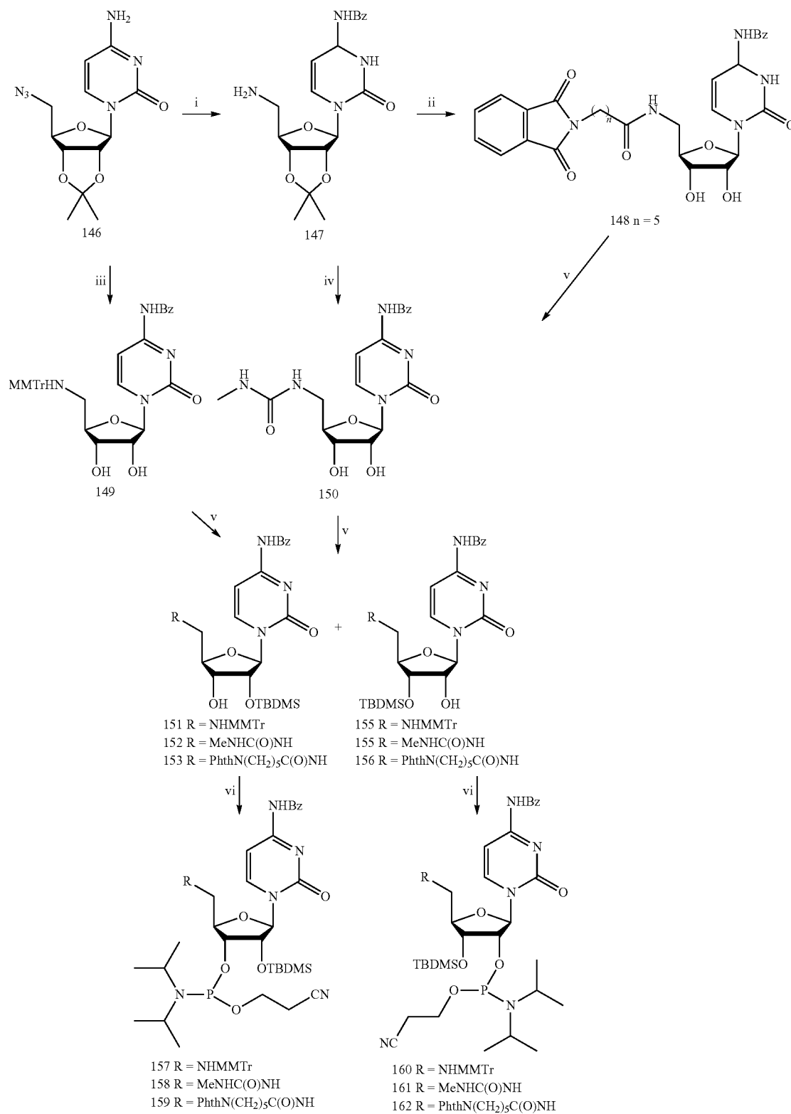
Scheme 7 a
