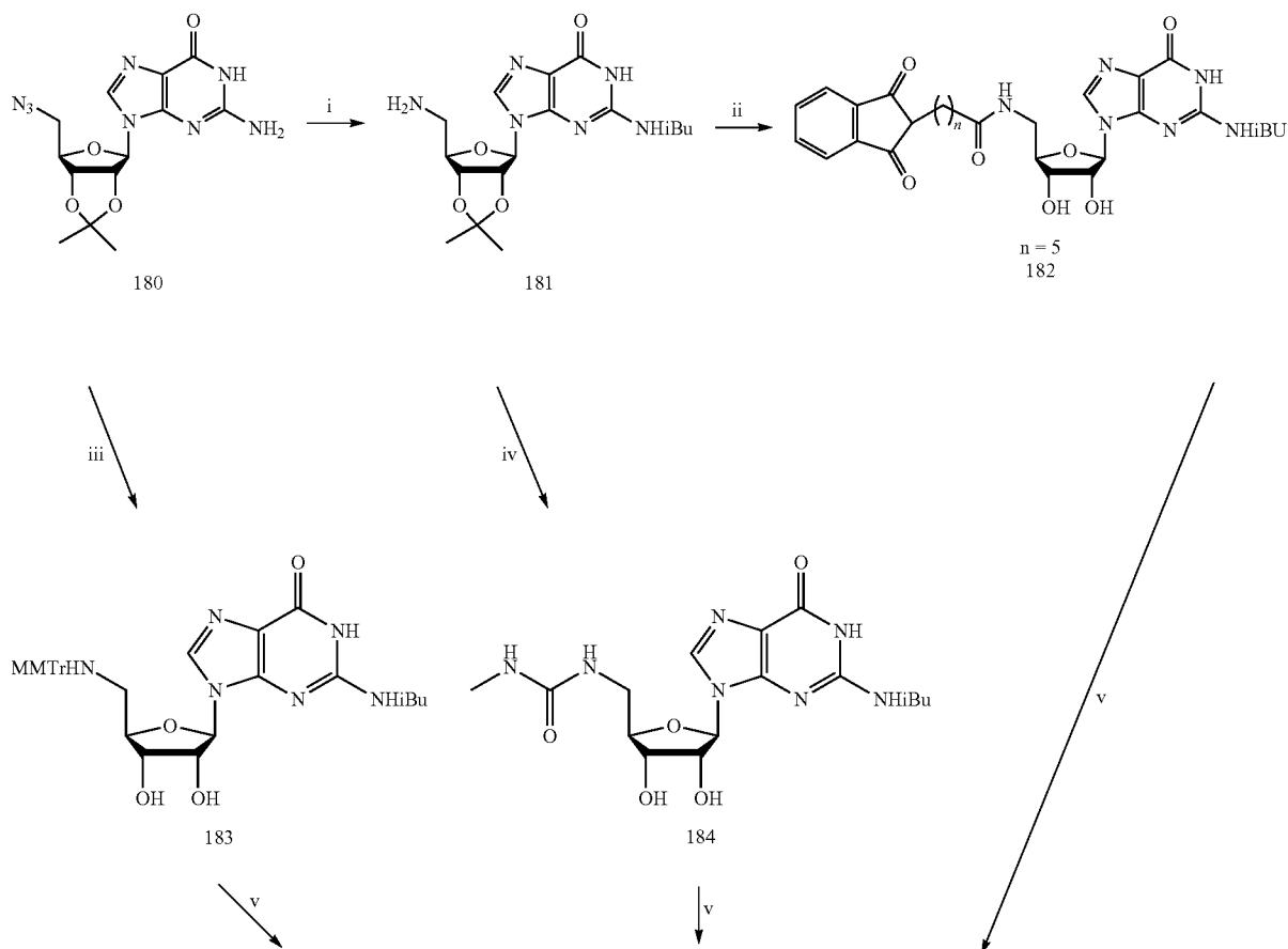
Scheme 9 a
