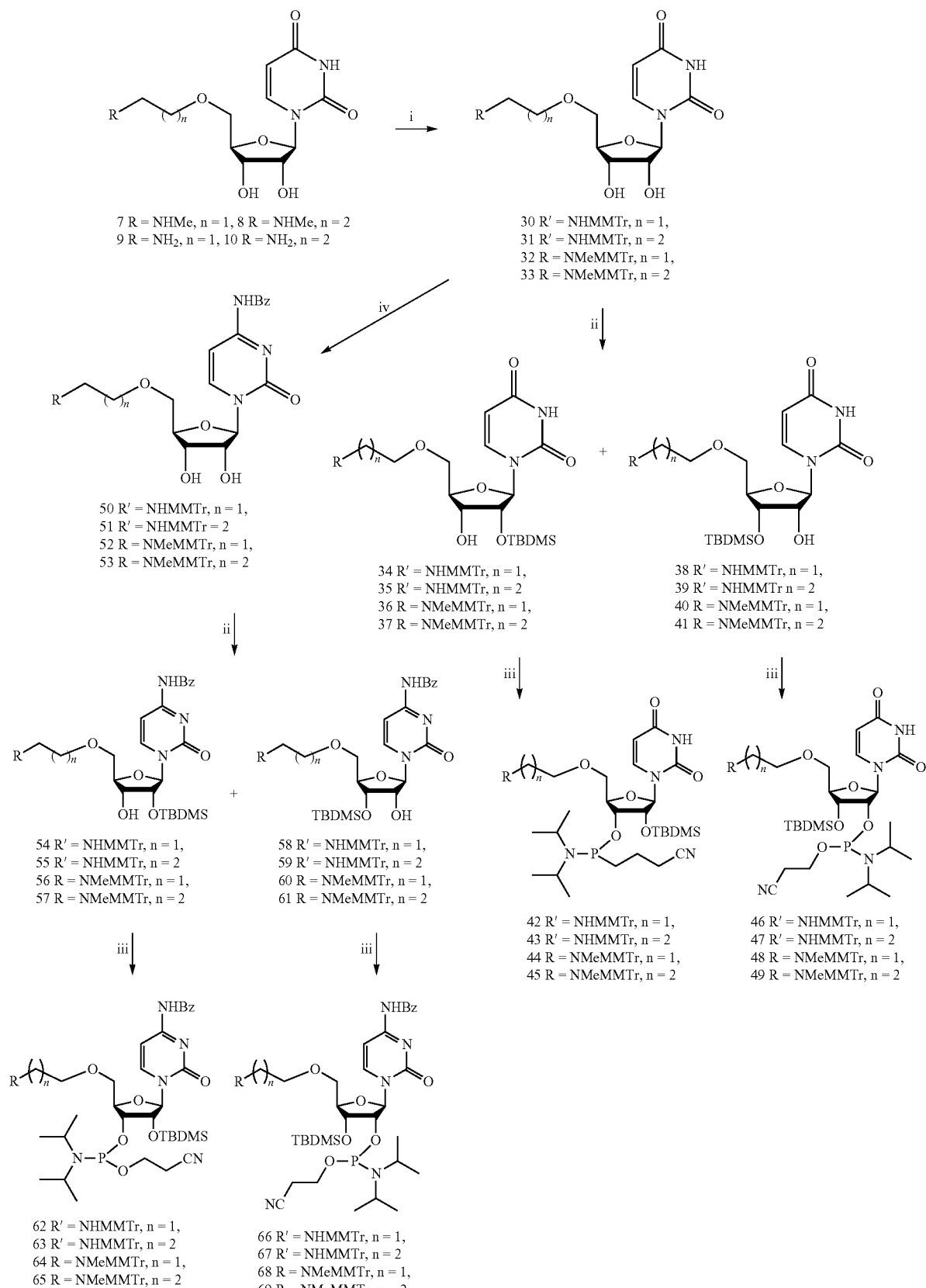
Scheme 2 a
