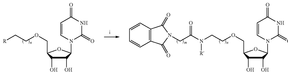
Scheme 4 a
