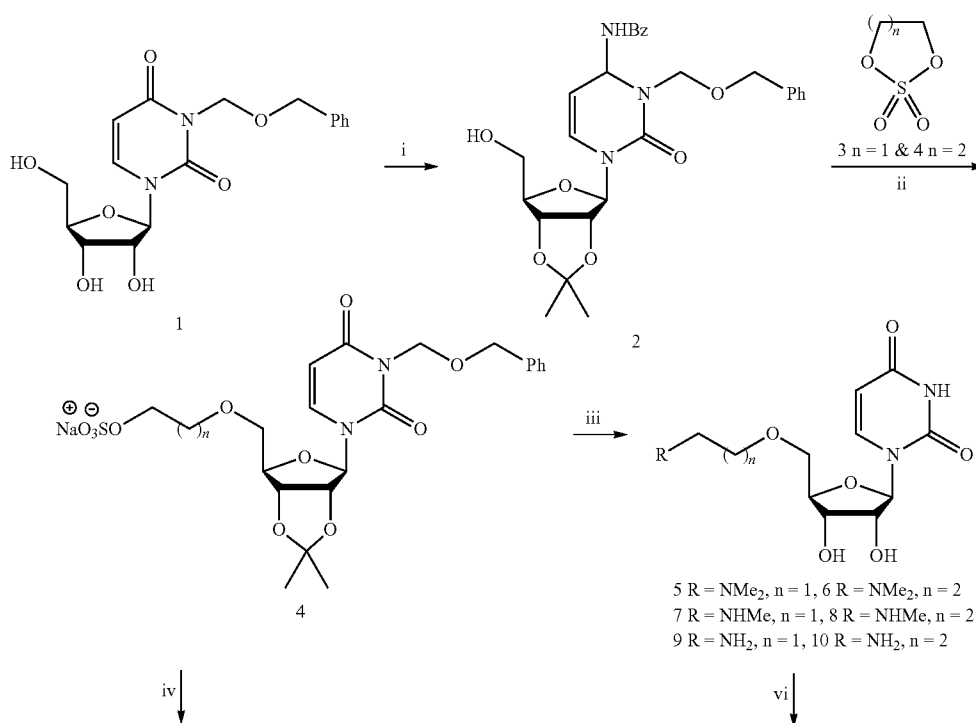
Scheme 1 a
