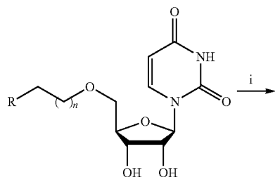
Scheme 3 a
