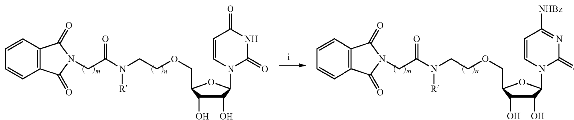
Scheme 5 a
