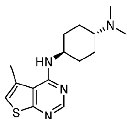
Cmp 4
