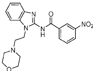
IRAK1/4 inhibitor
