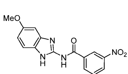
Compound 20
