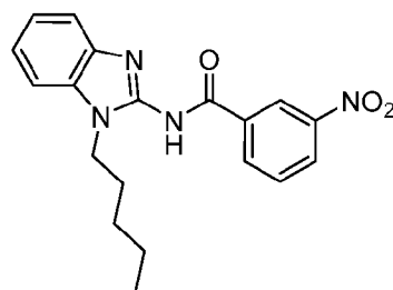
Compound 29
