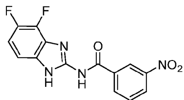
Compound 27
