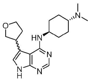
Cmp 19a/b
