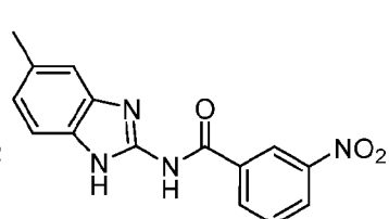
Compound 19
