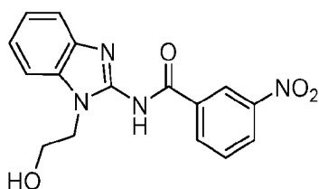
Compound 40
