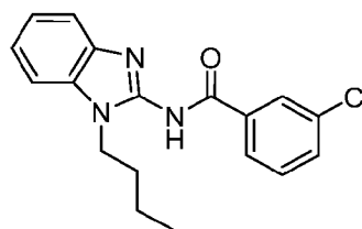
Compound 10
