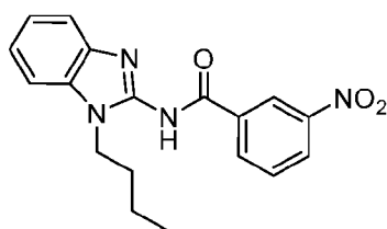
Compound 2
