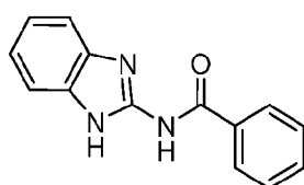
Compound 7
