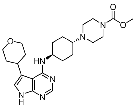
Cmp 27
