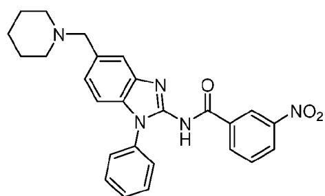
Compound 13
