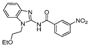
Compound 35
