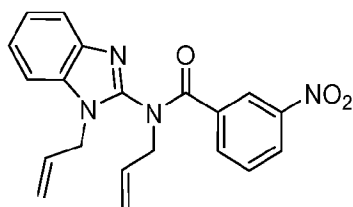
Compound 47
