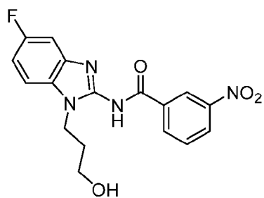
Compound 2
