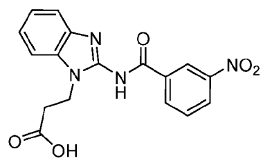
Compound 40
