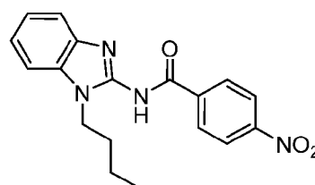
Compound 10
