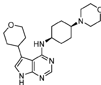
Cmp 32
