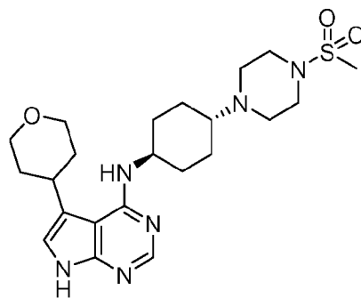
Cmp 26
