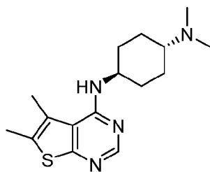
Cmp 2
