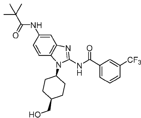
Compound 18
