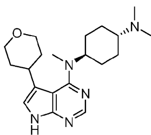
Cmp 22
