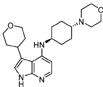
Cmp 35
