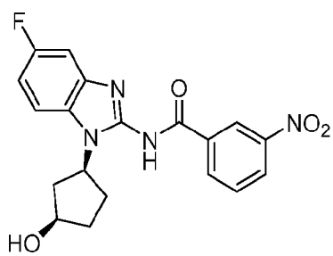
Compound 7
