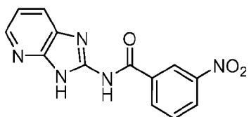
Compound 14
