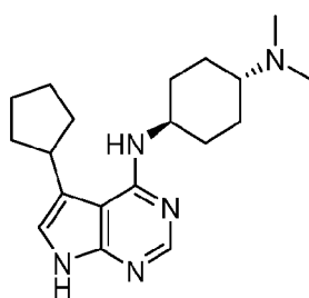
Cmp 17
