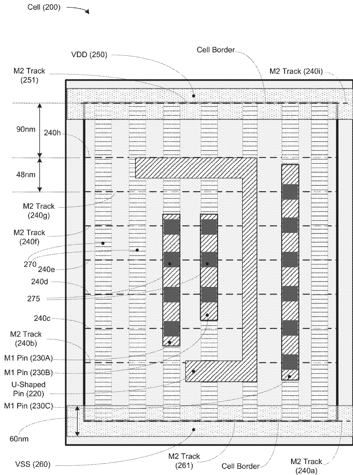
Fig. 2 (Prior Art)
