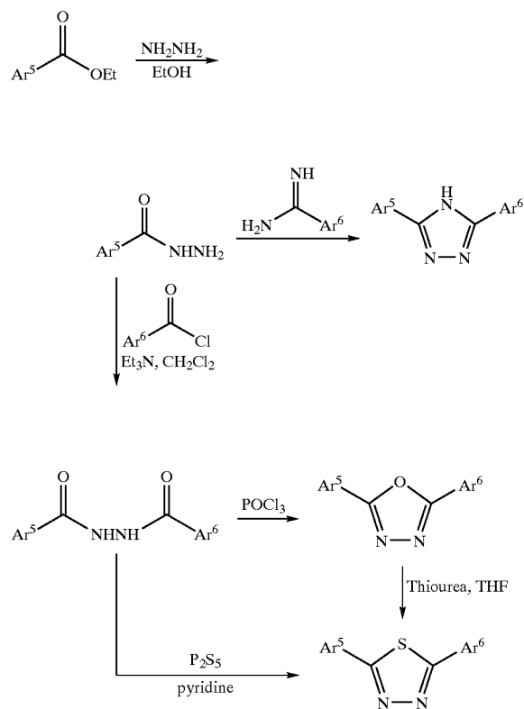
Reaction Scheme 3
