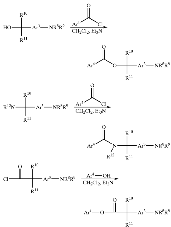
Reaction Scheme 2
