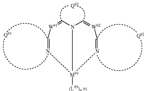
Formula (5-A)
