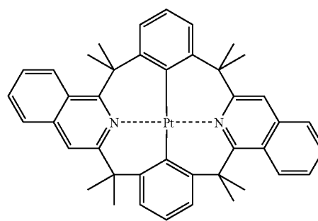
Compound (148)
