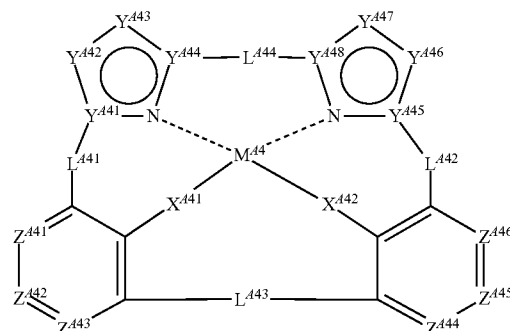
Formula (A-4)
