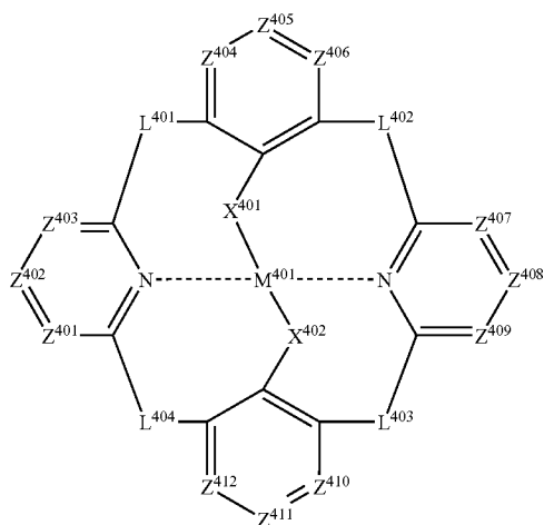
Formula (f)
