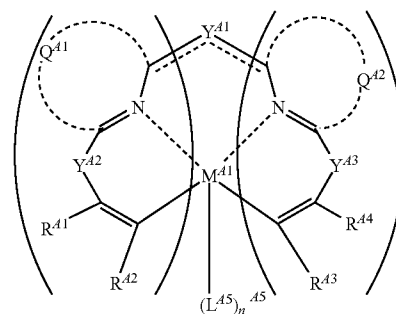
Formula (2) 55
