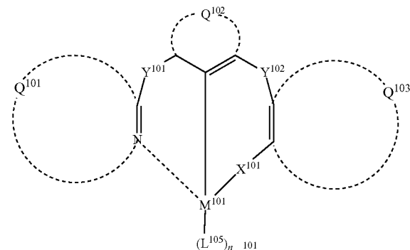
Formula (5-B)
