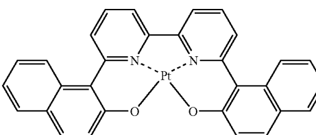
Compound (21)
