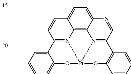
Compound (194)
