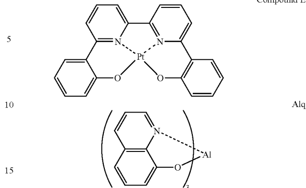
Compound E
