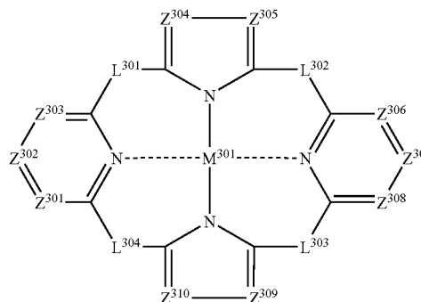
Formula (e)
