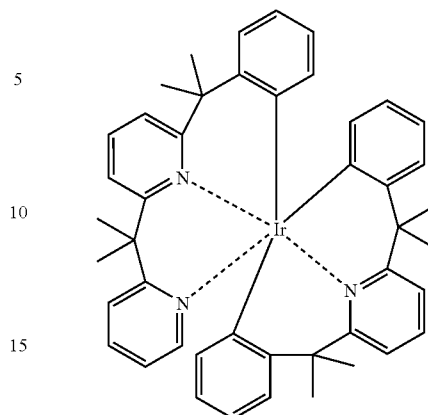
Compound (99)
