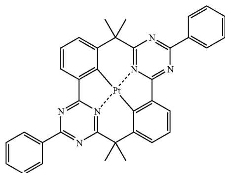
Compound (108)
