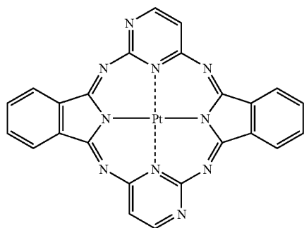
Compound (16)
