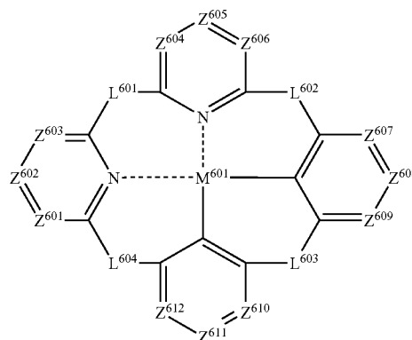
Formula (h)
