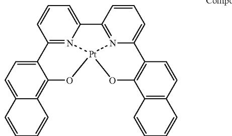
Compound (24)
