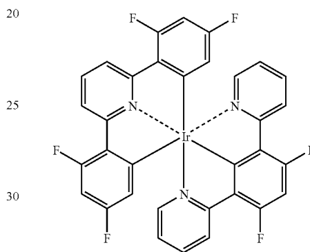
Compound (103)
