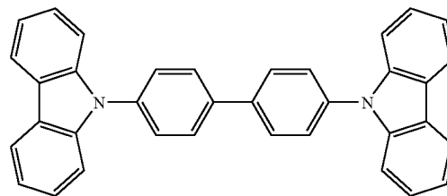
Compound B
