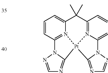
Compound (207)
