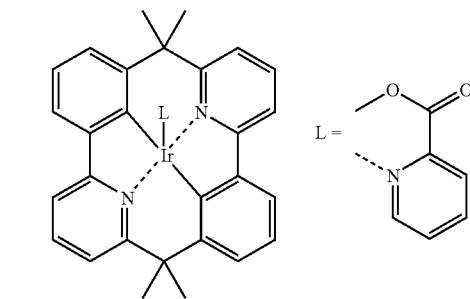
Compound (114)
