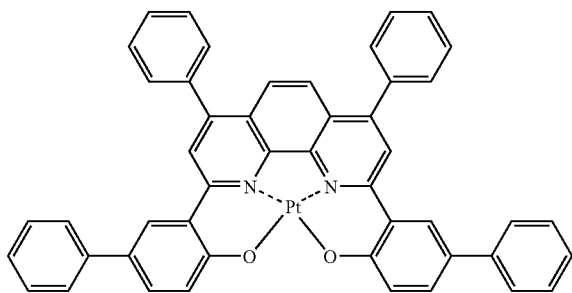
Compound (17)
