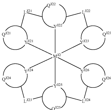
Formula (X2)
