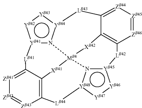
Formula (B-4)
