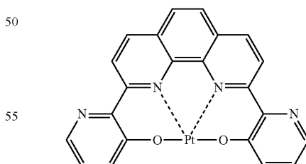
Compound (198)
