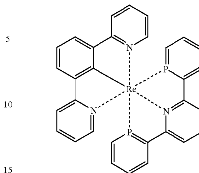
Compound (164)
