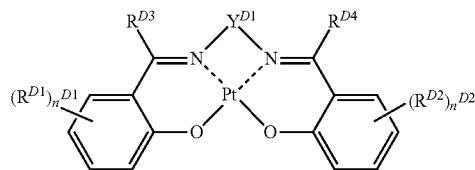
Formula (4-A)
