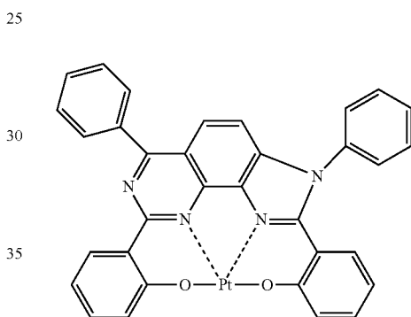
Compound (195)
