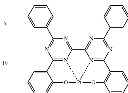
Compound (199)
