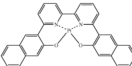
Compound (22)
