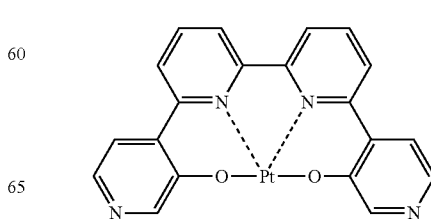
Compound (204)
