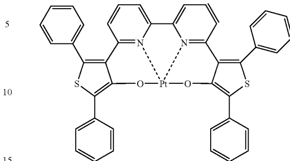
Compound (210)
