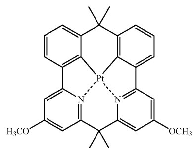
Compound (109)
