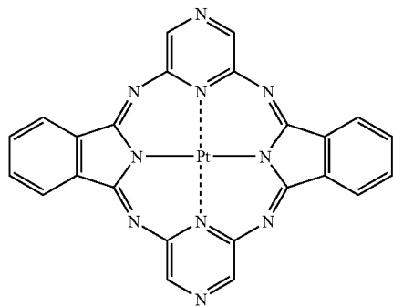
Compound (15)
