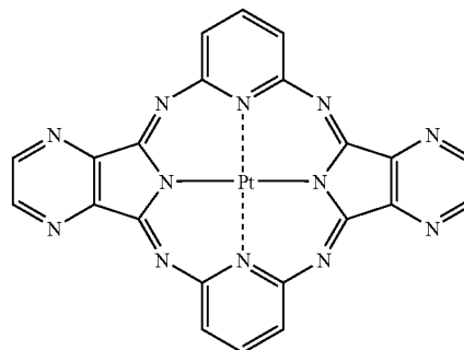
Compound (19)
