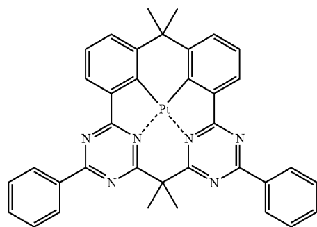
Compound (109)
