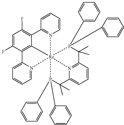
Compound (165)
