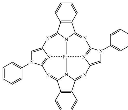
Formula (E-2)
