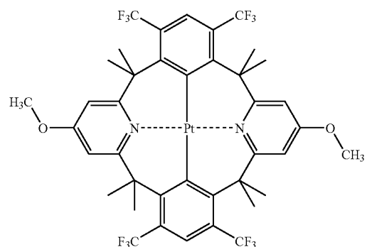
Compound (146)
