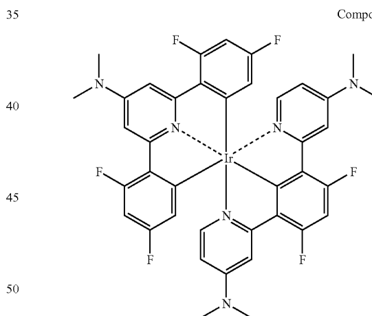
Compound (105)
