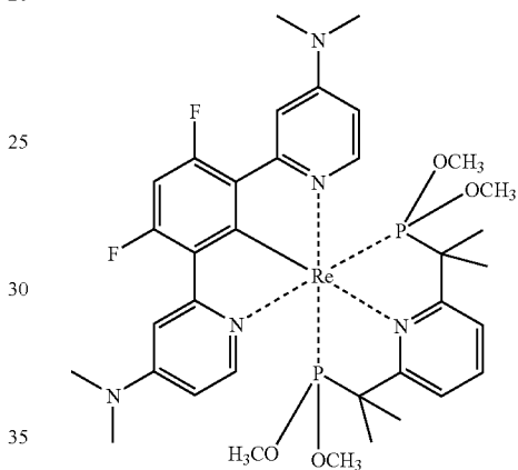
Compound (165)
