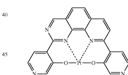
Compound (197)
