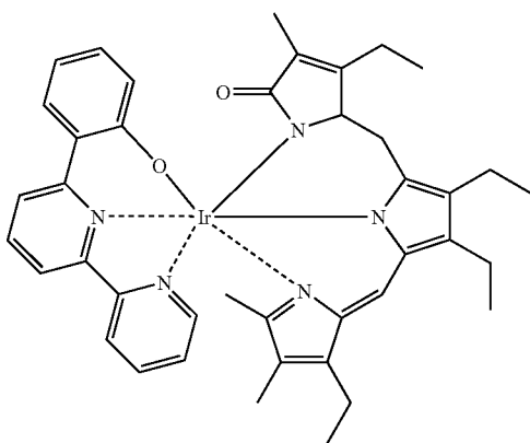
Compound (148)
