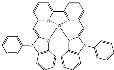
Compound (29)
