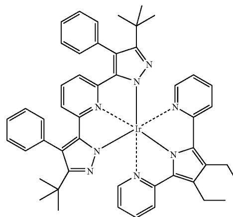
Compound (154)
