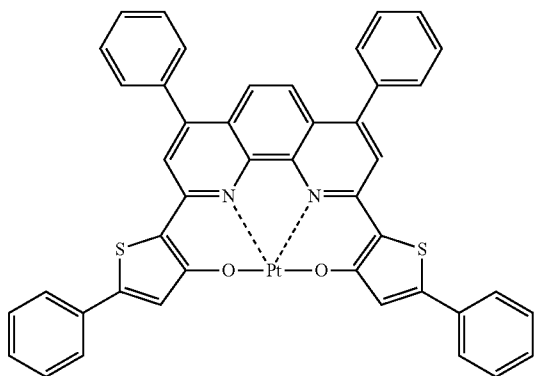
Compound (207)
