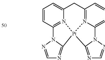
Compound (208)
