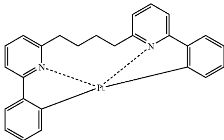
Compound (242)
