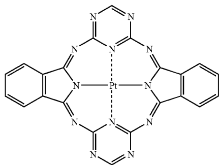
Compound (17)
