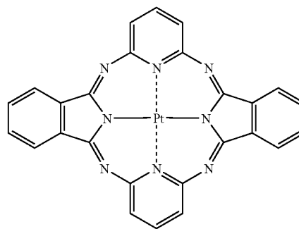
Compound (27)
