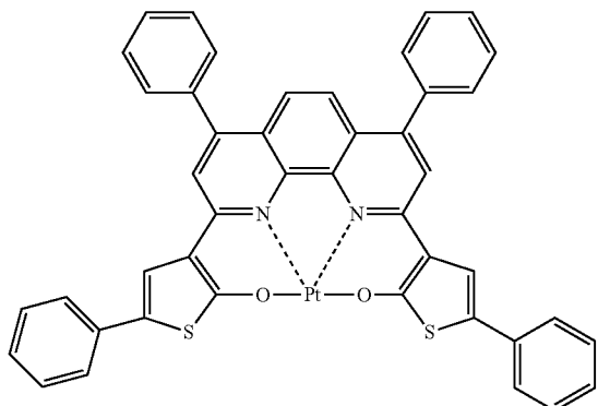
Compound (206)
