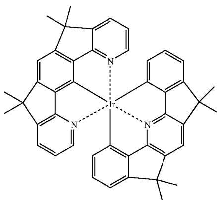
Compound (99)
