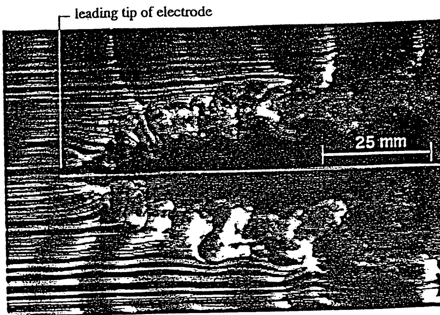
Figure 6(cont.) (c). Horizontal smoke wire flow visualization of a single electrode with symmetric plasma formation. The wire is at Y=2 mm. Stream velocity is 4 m/s.
