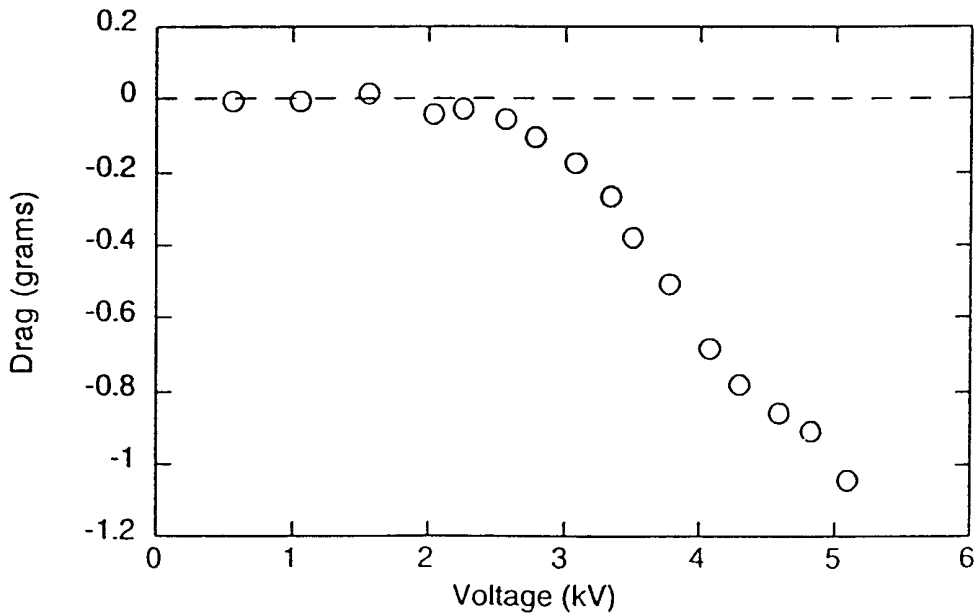
Figure 12. Electrostatic drag for panel E6-C in still air. Electrodes are spanwise, asymmetric with lower electrode staggered downstream relative to the upper electrode. Frequency: 3 kHz. Negative values correspond to a reduction in drag.
