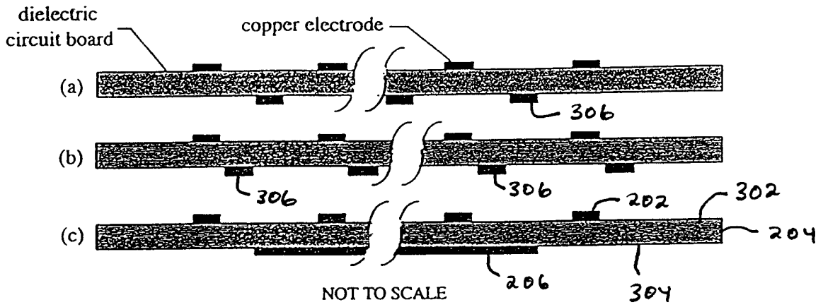
Figure 3 (a-c). Cross-sectional sketch of plasma panel concepts. (a) symmetric, staggered lower electrodes, (b) asymmetric, staggered lower electrodes, (c) symmetric, planar lower electrode
