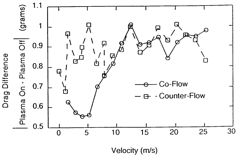
Figure 14. Drag change due to OAUGDP for panel E6-C in Co-flow and Counter-flow configurations (See Figure 13). Voltage and frequency were 4kV rms and 3kHz respectively.
