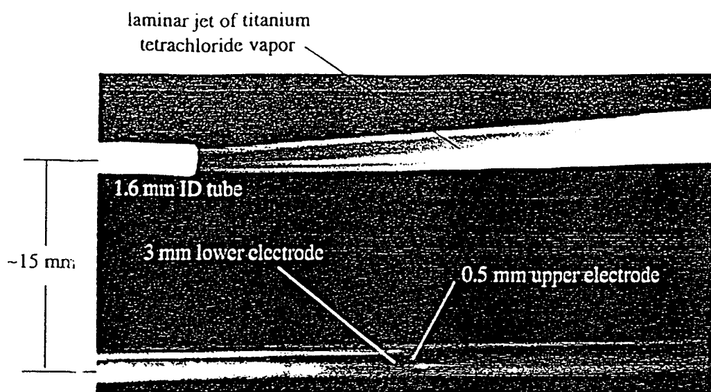
(a) Plasma Off
