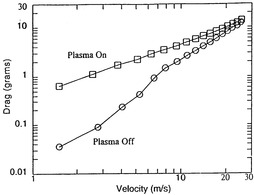
Figure 5a. Directly measured drag of panel C7-A (streamwise oriented electrodes) operated at 3.0 kHz and approx. 4.0 kV rms.
