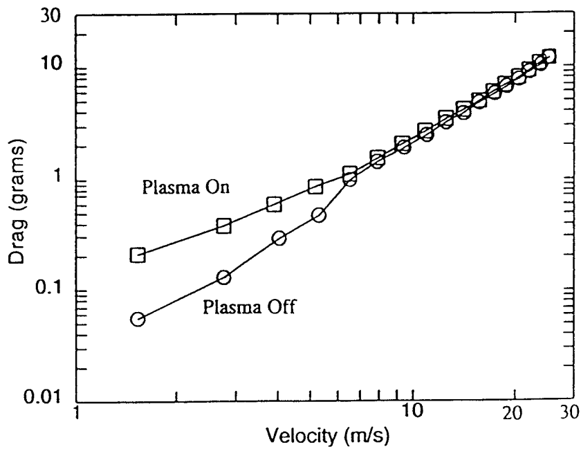
Figure 5b. Directly measured drag of panel C7-C (spanwise oriented electrodes) operated at 3.0 kHz and approx. 4.0 kV rms.
