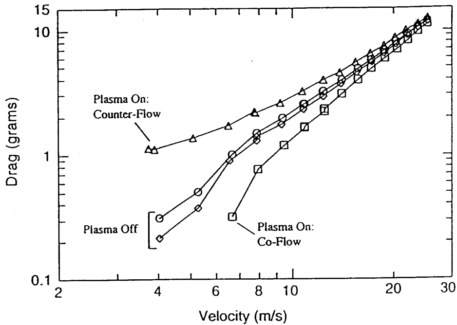
Figure 13. Directly measured drag of panel E6-C (spanwise, asymmetric electrodes, 4 kV, 3 kHz). Co-flow case corresponds to bottom electrode staggered downstream of top electrode; Counter-flow corresponds bottom electrode staggered upstream of top electrode.
