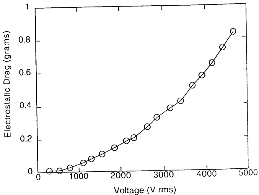
Figure 7. Electrostatic drag for panel C1-B (staggered upper electrodes over planar lower electrode); F=1.5 kHz, U_{\infty}=0 .
