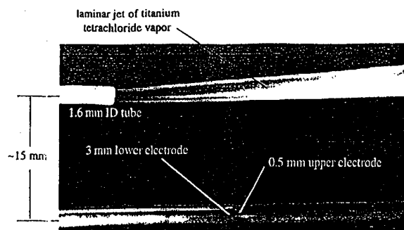
(a) Plasma Off
