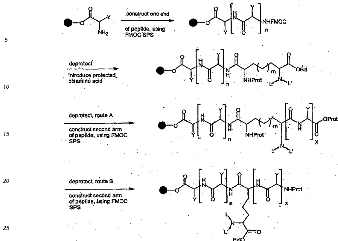
Scheme 4. Integration of the bifunctional chelate into the peptide sequence.
