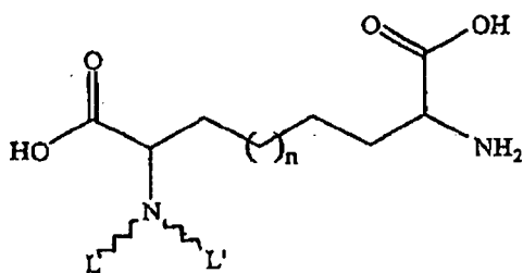
Scheme 3. The amino acid-based bifunctional chelates of this study.
