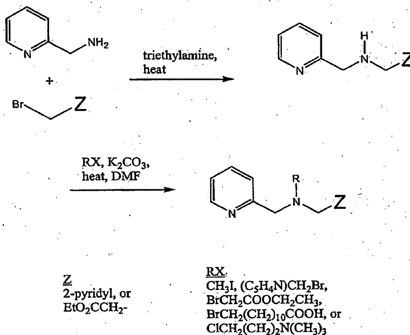
Scheme 1. Synthesis of various DPMA derivatives.
