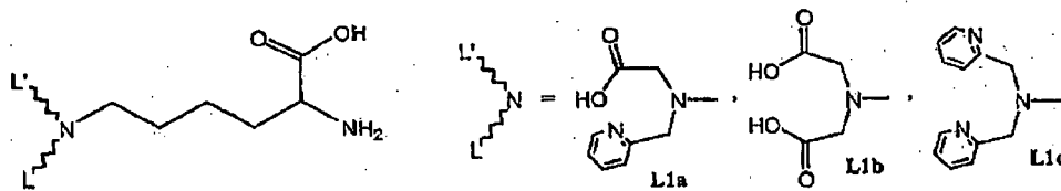
\epsilon -derivatized lysine, L1
