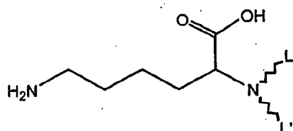
\alpha -derivatized lysine, L2
