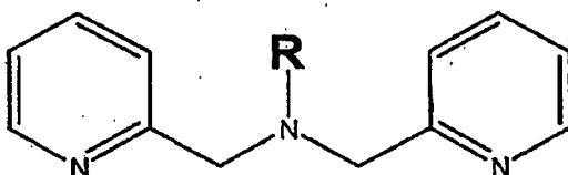
R = biologically relevant molecule
