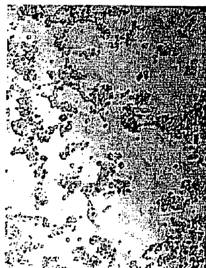
T7 siRNA
