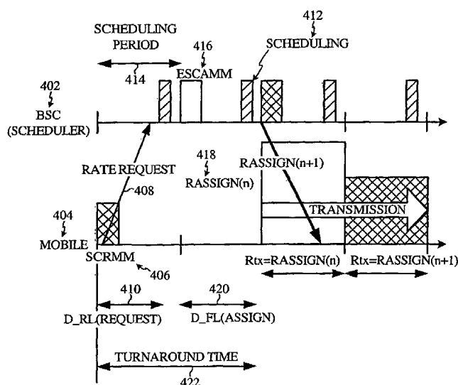
PARAMETERS ASSOCIATED IN MOBILE STATION SCHEDULING ON RL
