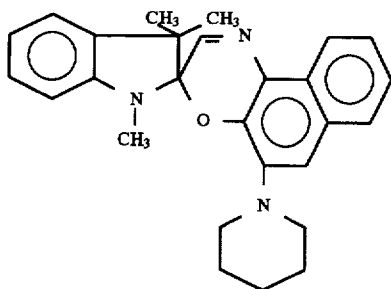
1,3,3-Trimethylspiro(indolino-6'-(1-piperidyl)-2,3'-(3H)naphtho-2,1b)(1,4)oxazine
