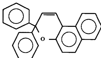
3,3-Diphenyl-3H-naphtho(2,1b)pyran
