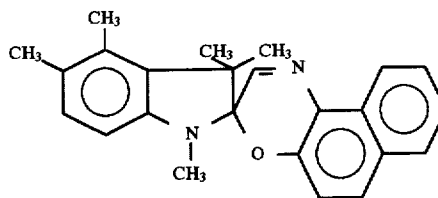
1,3,3,5,6-pentamethylspiro(indolino-2,3'-[3H]naphtho(2,1b)-(1,4)oxazine)
