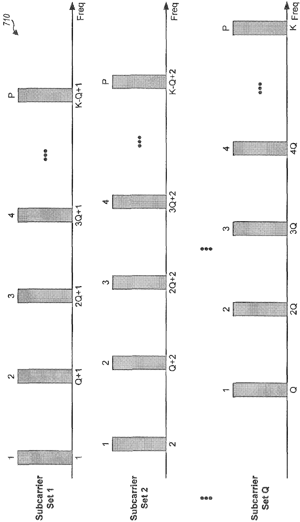
Subcarrier FIG. 7B
