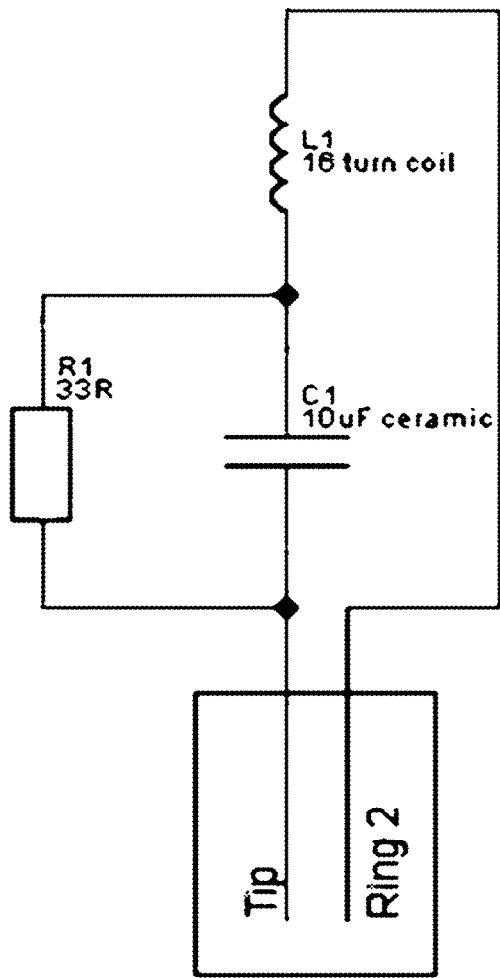
TRRS 4-way jack socket Fig. 1
