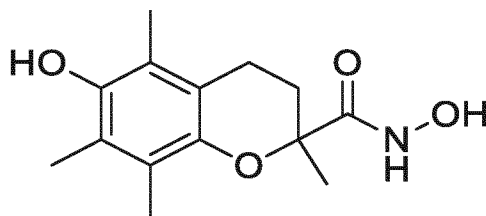
N,6-dihydroxy-2,5,7,8-tetramethylchroman-2-carboxamide (III)
