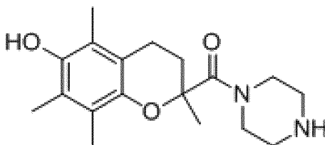
(6-hydroxy-2,5,7,8-tetramethylchroman-2-yl)(piperazin-1-yl)methanone (II)
