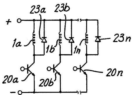
FIG. 2 PRIOR ART
