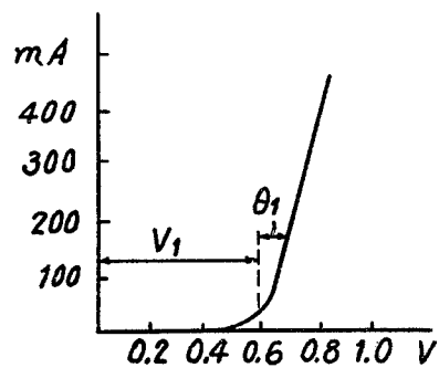
FIG. 3 PRIOR ART
