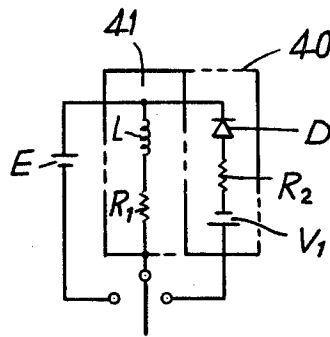
FIG. 5 PRIOR ART
