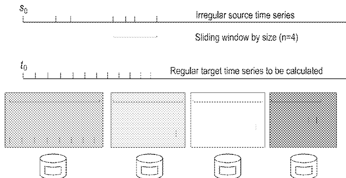
Time alignment with MapReduce
