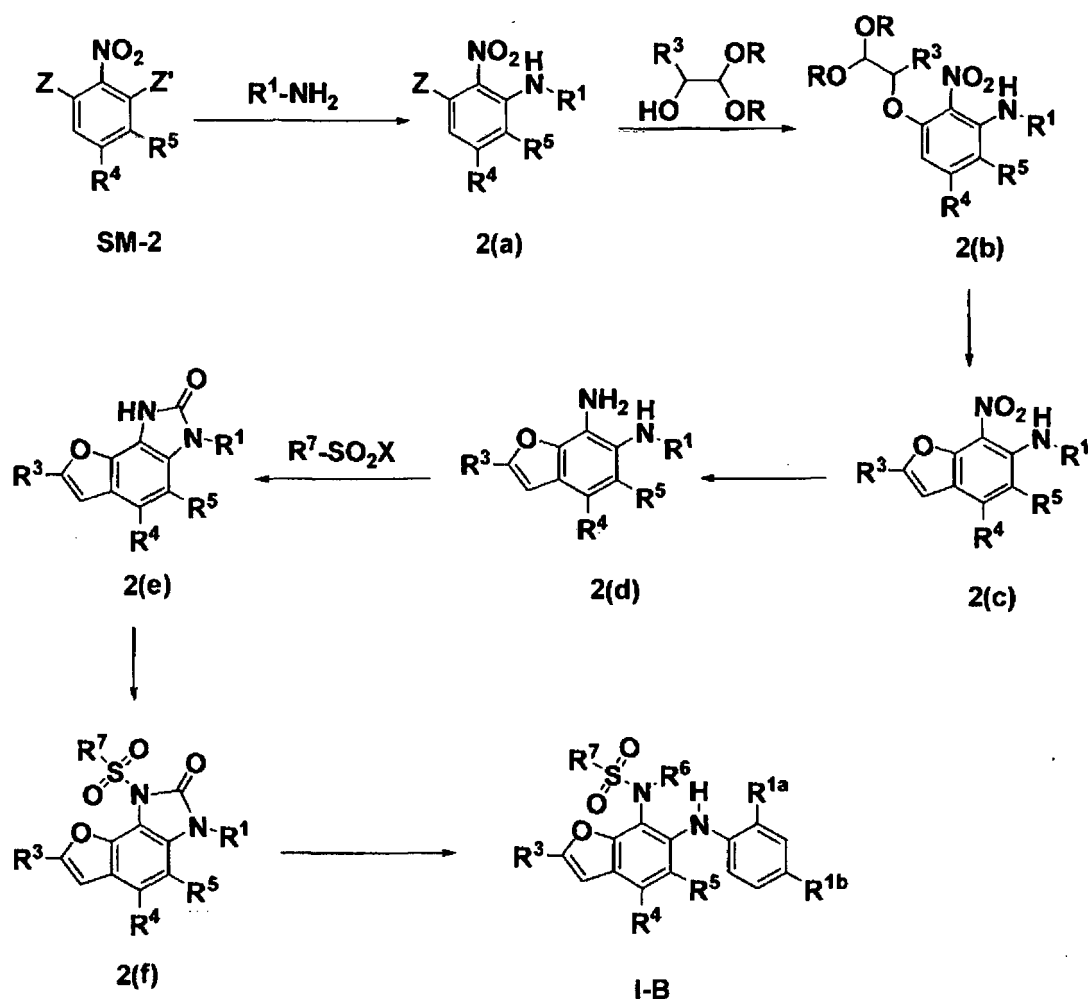
Scheme II
