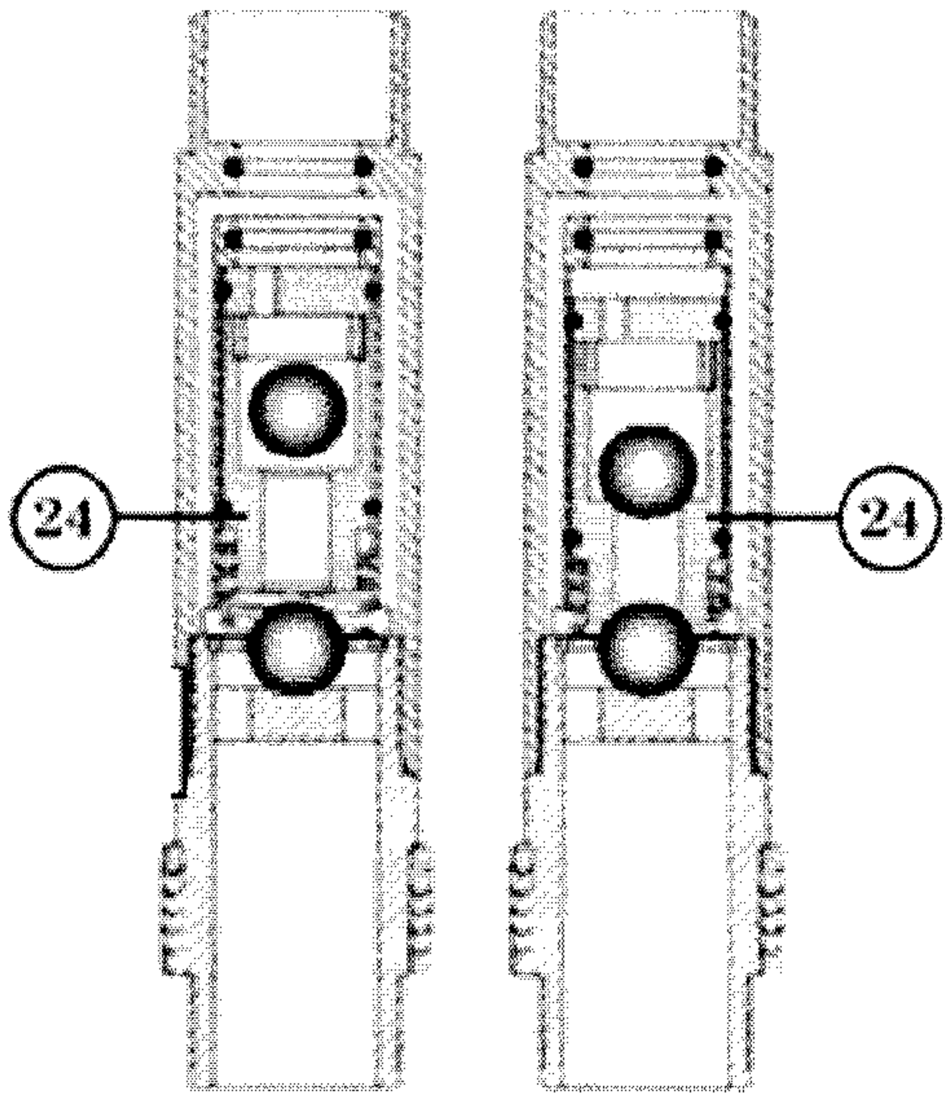
Position of plunger (24) in the opening And closing of bottom valve
