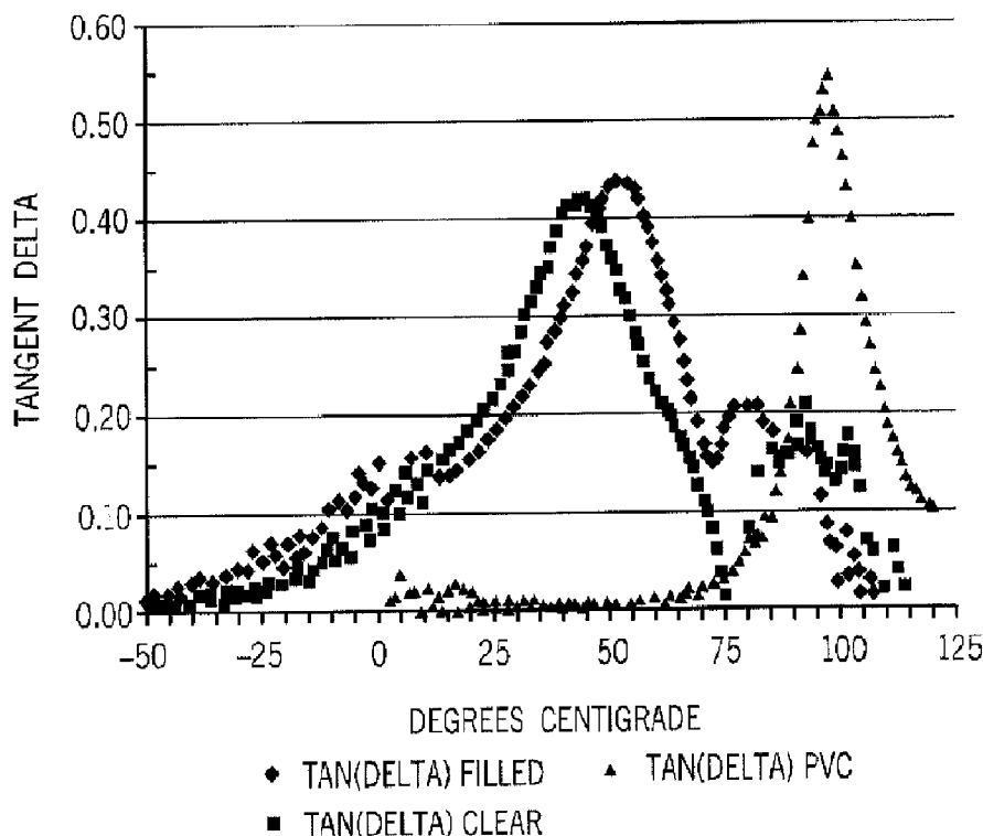
1Hz DMA ALGAE EPOXY IN PVC VERSUS PURE PVC
