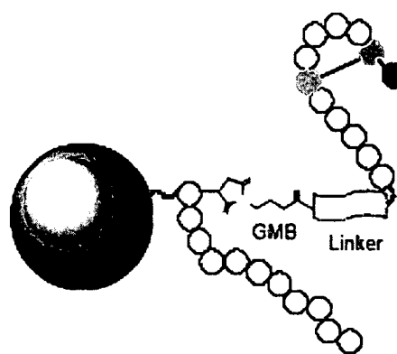
KLH-(301-311)-Li-(E-c421-433)
