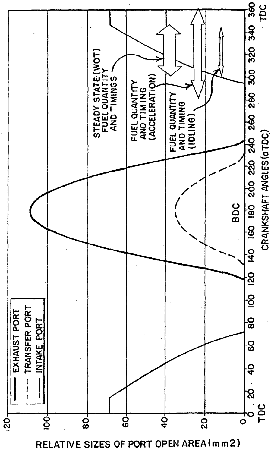
FIG. 9 PISTON PORT AND ROTARY VALVE CONTROLLED INTAKE SYSTEM
