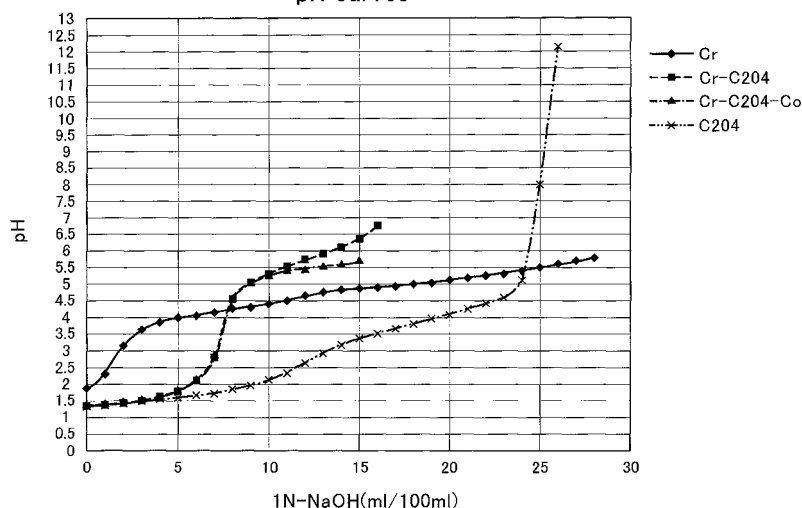
FIG.1 pH curves
