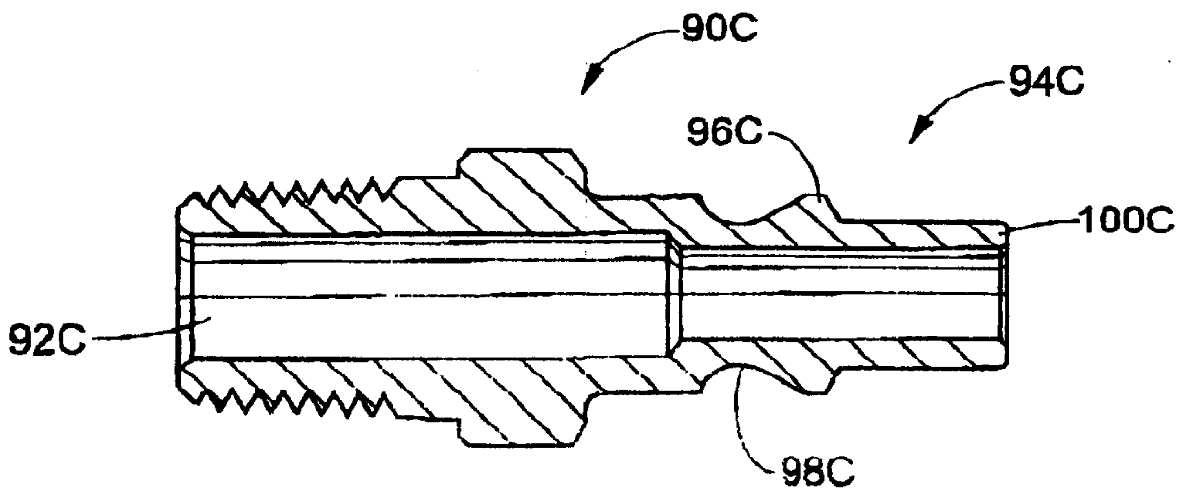
FIG. 6C (PRIOR ART)
