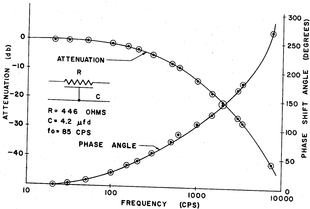
ATTENUATION AND PHASE ANGLE VERSUS FREQUENCY MEASURED ON TANTALUM DISTRIBUTED COMPONENT
