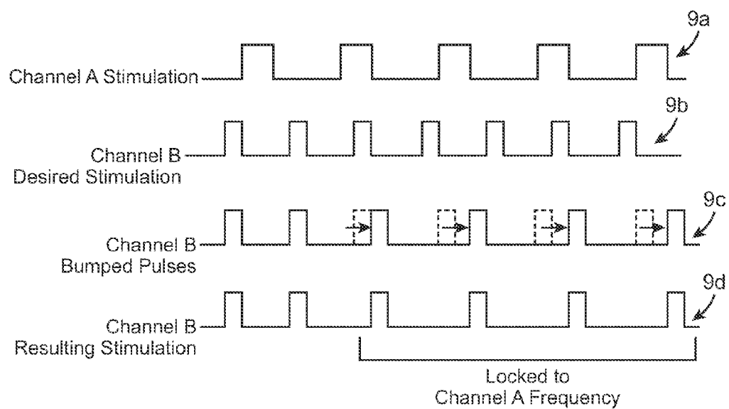
FIG. 4 (PRIOR ART)
