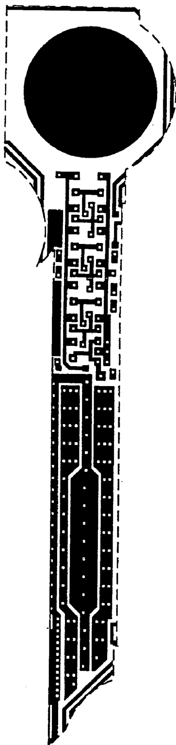
Metal 1 mask
