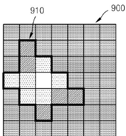
METABOLITE MAP
