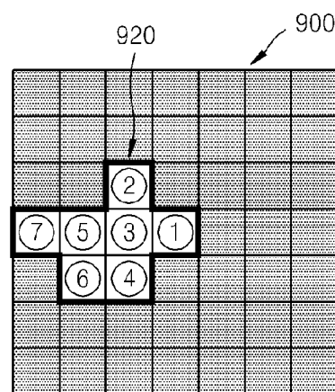
METABOLITE MASK
