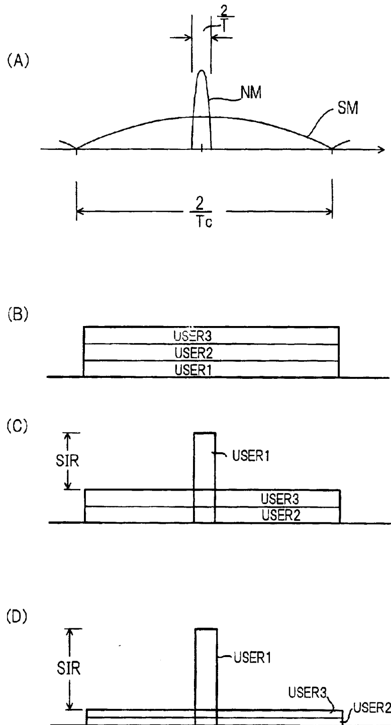
FIG. 16 PRIOR ART
