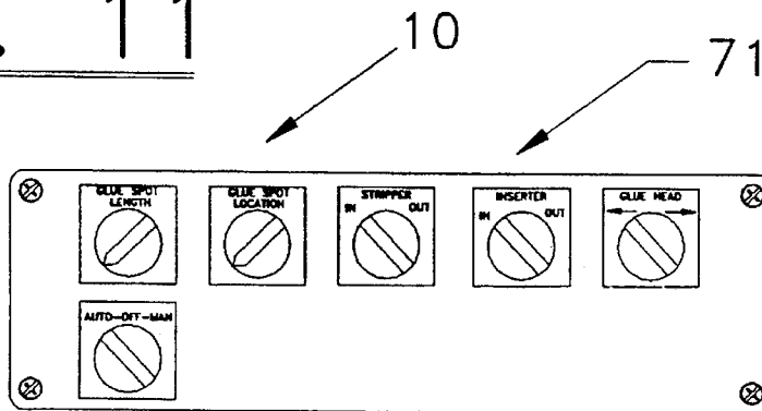
SET-UP PANEL
