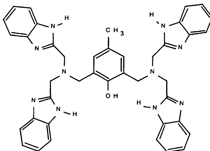
N,N,N',N'-Tetrakis-(2-benzimidazolymethyl)-2-hydroxy-1,3-diaminopropan,
