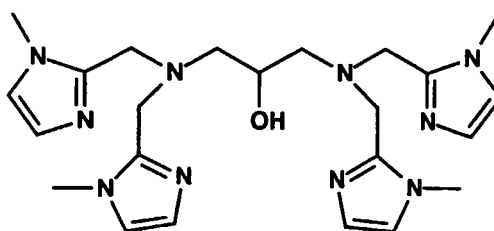
N,N,N',N'-Tetrakis[2-(1-methyl)-imidazolymethyl]-1,3-diamino-2-propanol
