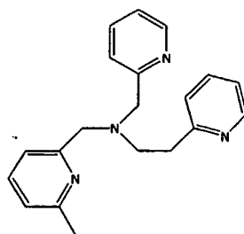
pmap [2-(2-pyridyl)ethyl][(2-pyridyl)methyl)][(6-methyl-2-pyridyl)-methyl]amin
