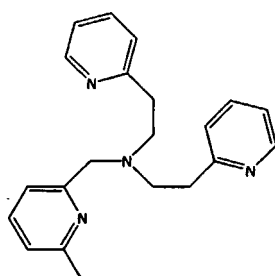
pmea [(2-pyridyl)methyl][2-(2-pyridyl)ethyl)][(6-methyl-2-pyridyl)-methyl]amin
