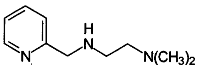
(2-Pyridylmethyl)(3-(N,N-dimethylamino)-propyl)amin
