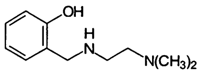
(2-Hydroxybenzyl)(2-(N,N-dimethylamino)-ethyl)amin
