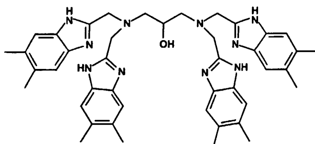
N,N',N'',N'''-Tetrakis[2-(5,6-dimethyl)-benzimidazolymethyl]-1,3-diamino-2-propanol
