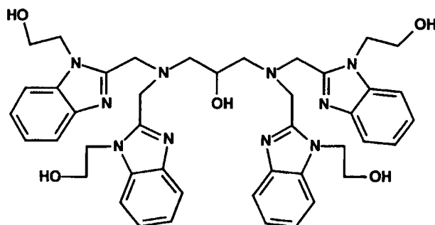
N,N,N',N'-Tetrakis[2-(2-hydroxyethyl)-benzimidazolymethyl]-1,3-diamino-2-propanol
