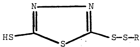
2-mercapto-5-hydrocarbyldithio-1,3,4-thiadiazole
