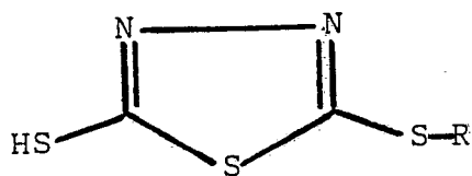
2-mercapto-5-hydrocarbylthio-1,3,4-thiadiazole
