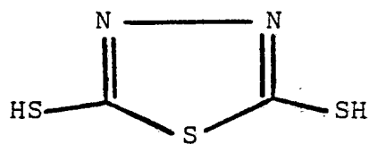
2,5-dimercapto-1,3,4-thiadiazole
