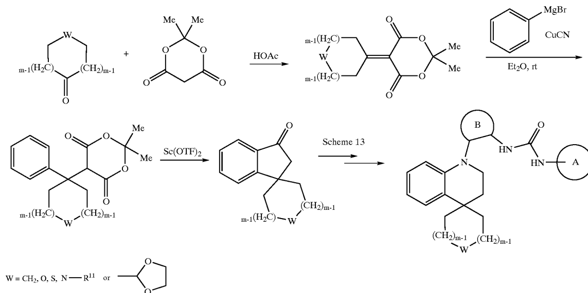
Scheme 18
