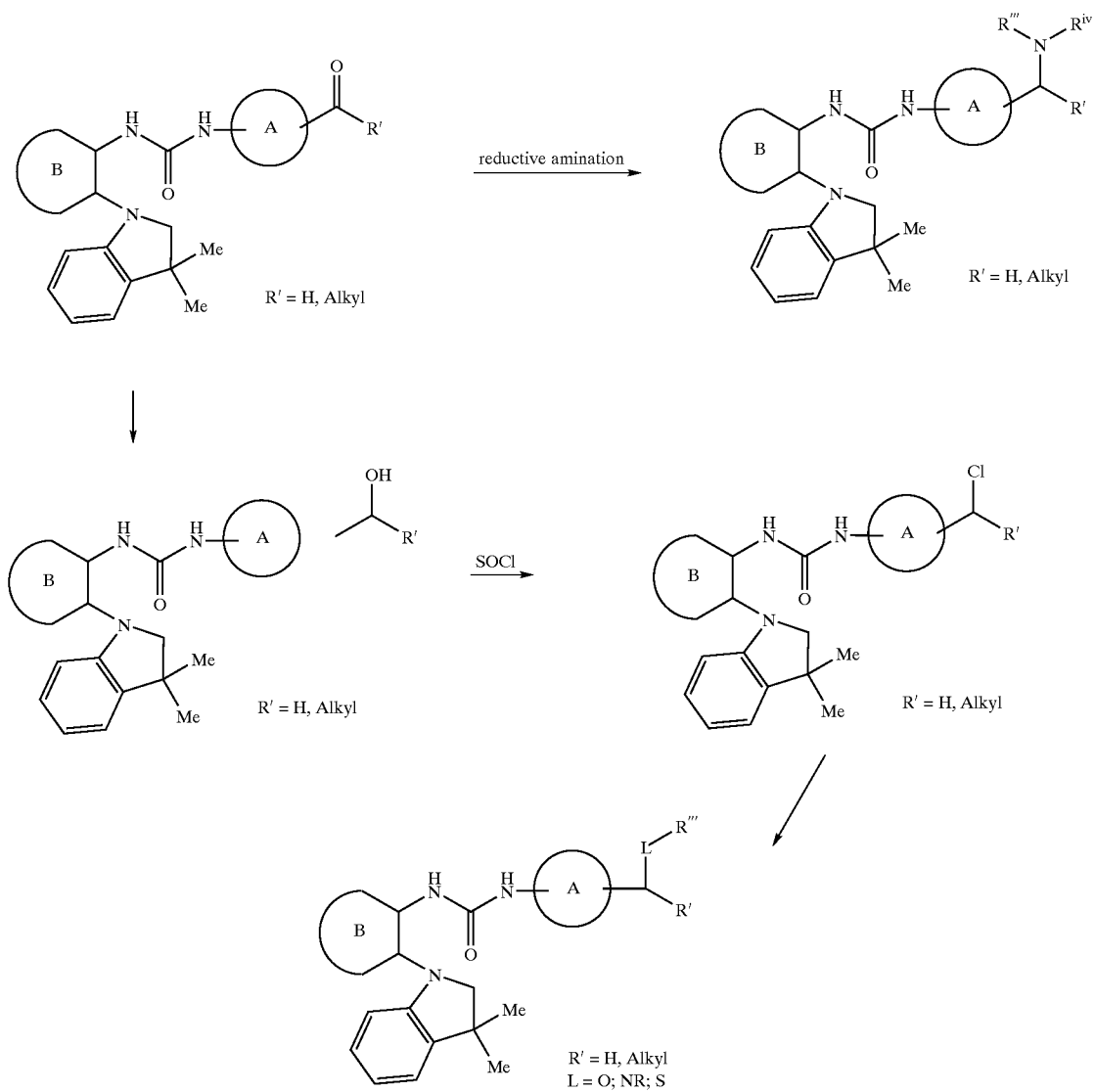
Scheme 13
