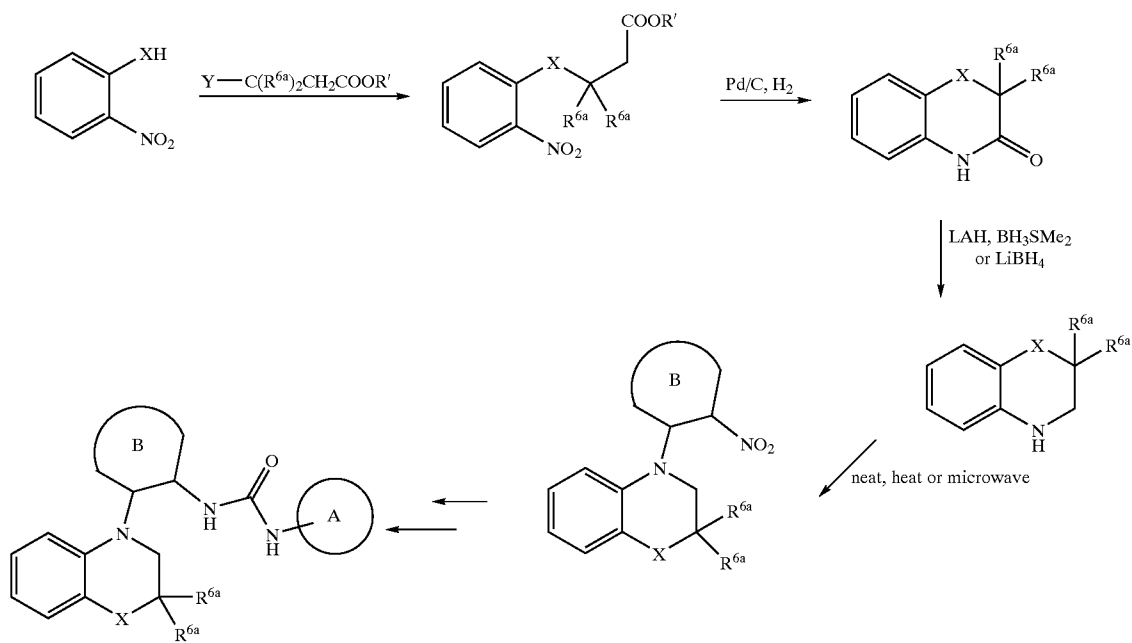
Scheme 15
