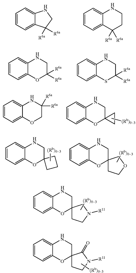
Scheme 10
