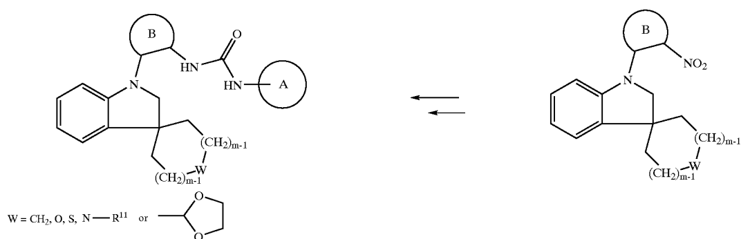
Scheme 18
