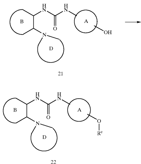
Scheme 9
