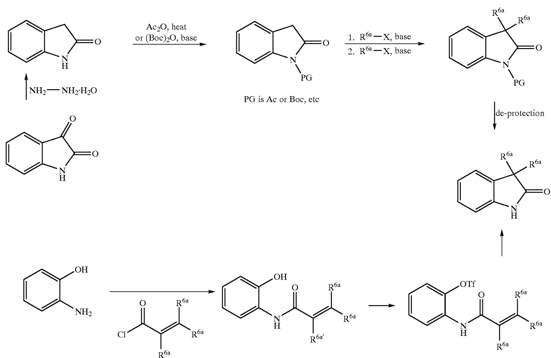
Scheme 12
