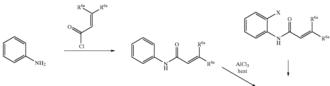
Scheme 14
