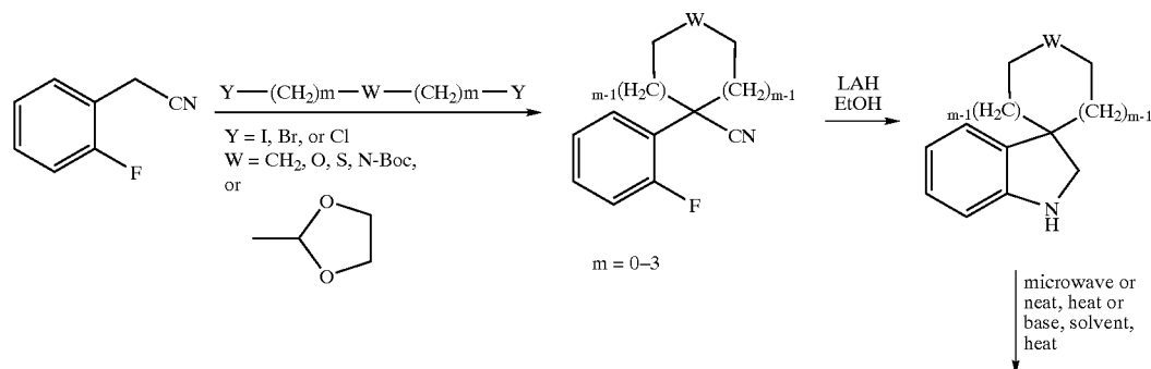
Scheme 17
