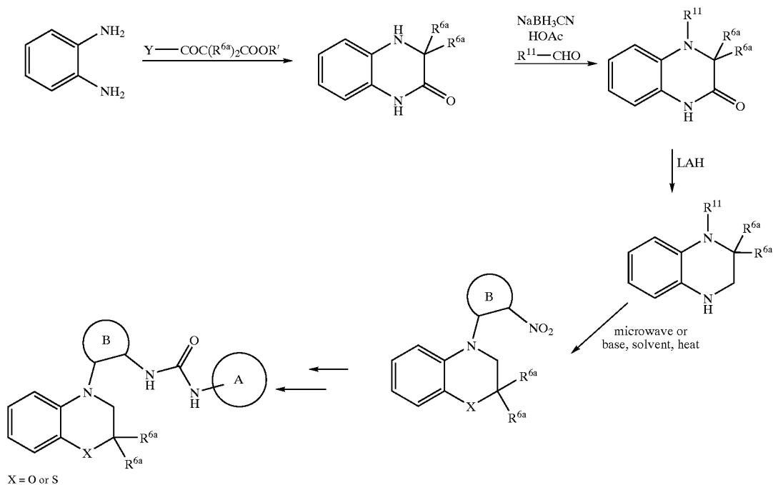
Scheme 16
