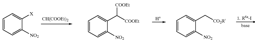
Scheme 11
