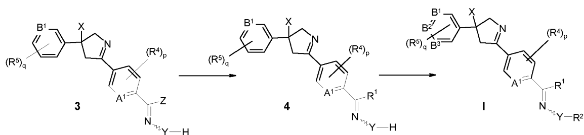
Scheme 2
