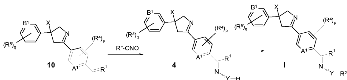
15 Scheme 7
