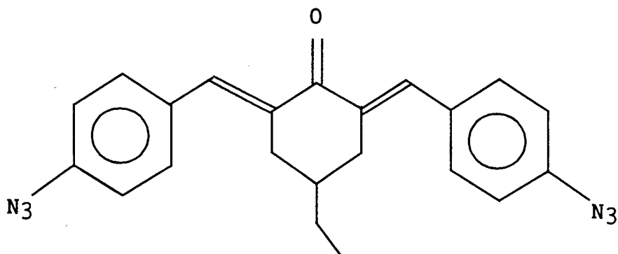
2,6-bis(4-azidobenzylidene)-4-ethylcyclohexanone (BAC-E)
