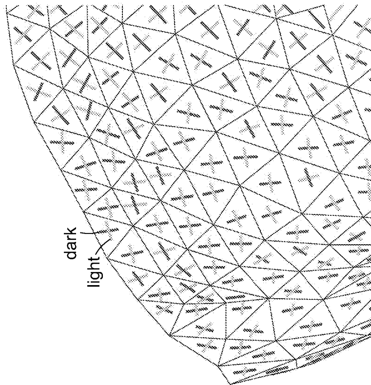
Detail A
